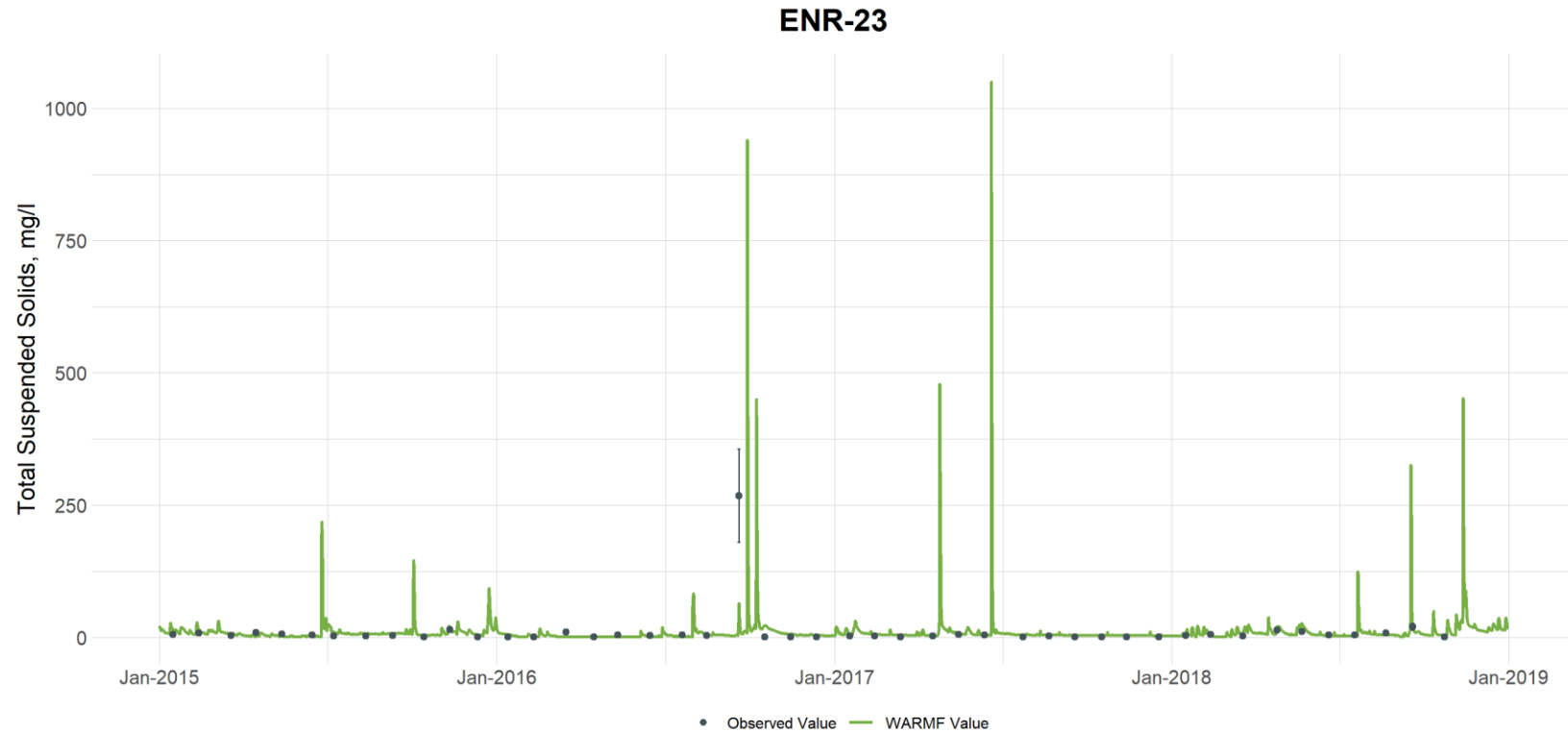
Figure G-23. Comparison of Observed and Simulated Total Suspended Solids (silt+clay) Concentrations at Eno River at Station ENR-23 (vertical bars are used to illustrate the uncertainty with laboratory analyses and are based on the 95th percentile confidence interval calculated from the UNRBA data set for each parameter)
