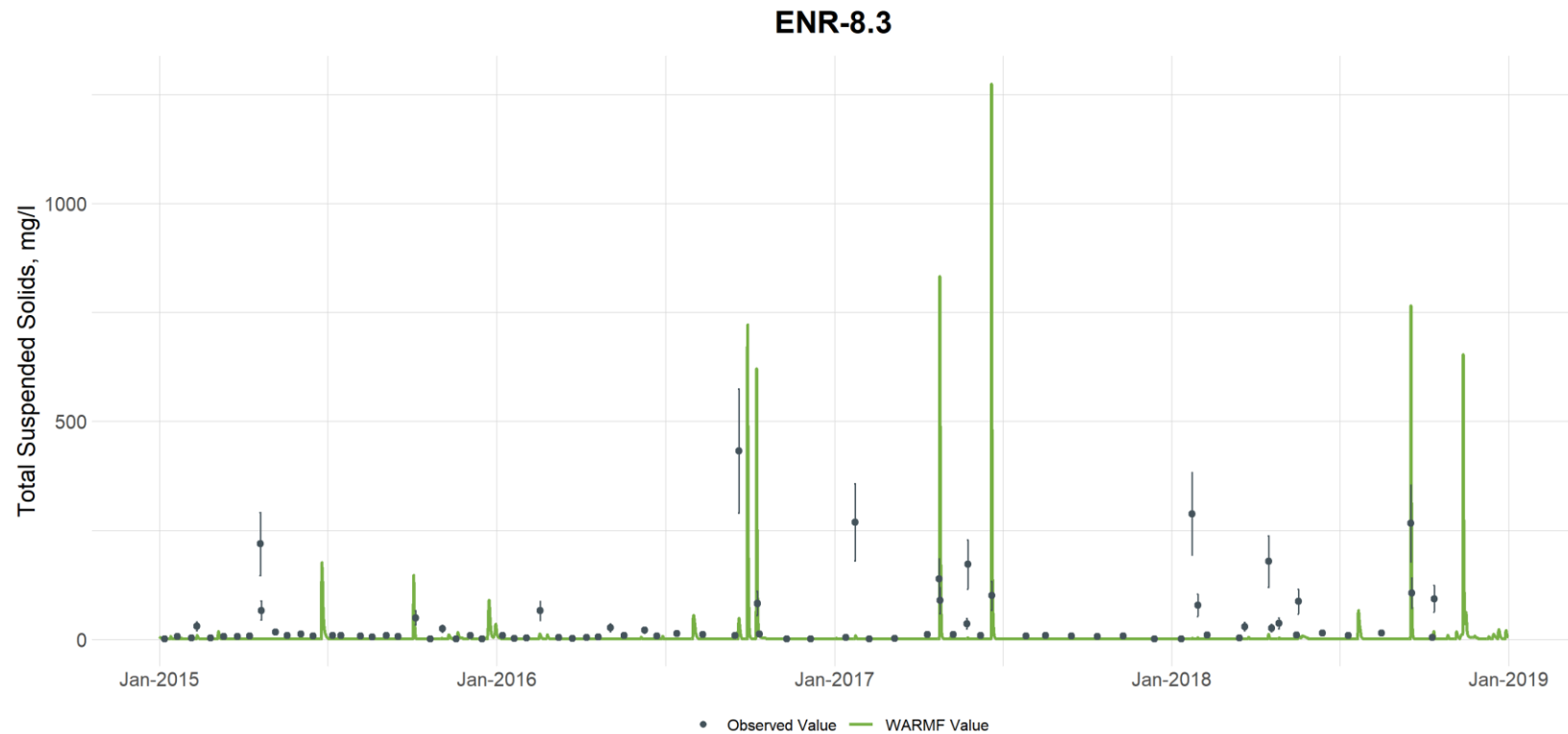
Figure G-32. Comparison of Observed and Simulated Total Suspended Solids (silt+clay) Concentrations at Eno River at Station ENR-8.3 (vertical bars are used to illustrate the uncertainty with laboratory analyses and are based on the 95 th percentile confidence interval calculated from the UNRBA data set for each parameter)
