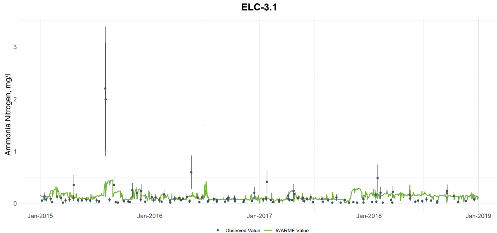
Figure G-5. Comparison of Observed and Simulated Ammonia Concentrations at Ellerbe Creek at Station ELC-3.1 (vertical bars are used to illustrate the uncertainty with laboratory analyses and are based on the 95th percentile confidence interval calculated from the UNRBA data set for each parameter)
