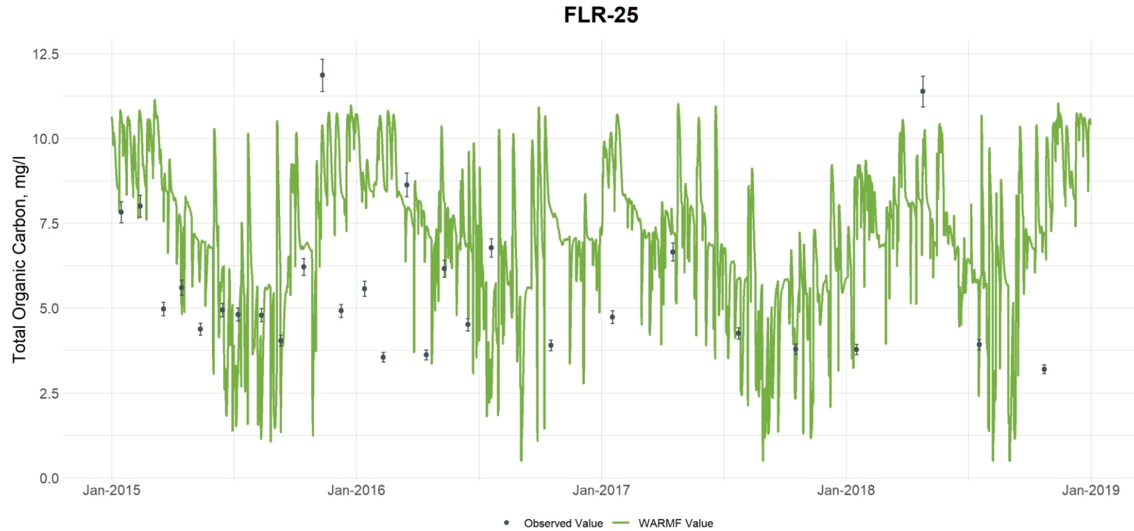
Figure G-41. Comparison of Observed and Simulated Total Organic Carbon Concentrations at Flat River at Station FLR-25 (vertical bars are used to illustrate the uncertainty with laboratory analyses and are based on the 95 th percentile confidence interval calculated from the UNRBA data set for each parameter)
