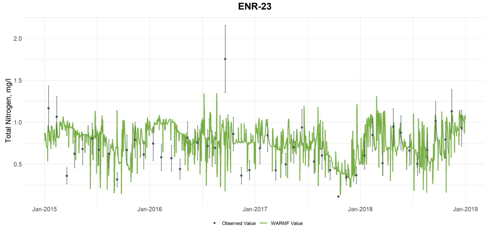
Figure G-20. Comparison of Observed and Simulated Total Nitrogen Concentrations at Eno River at Station ENR-23 (vertical bars are used to illustrate the uncertainty with laboratory analyses and are based on the 95th percentile confidence interval calculated from the UNRBA data set for each parameter)
