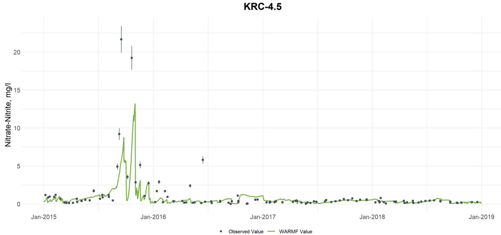
Figure G-57. Comparison of Observed and Simulated Nitrate-Nitrite Concentrations at Knap of Reeds Creek at Station KRC-4.5 (vertical bars are used to illustrate the uncertainty with laboratory analyses and are based on the 95th percentile confidence interval calculated from the UNRBA data set for each parameter)
