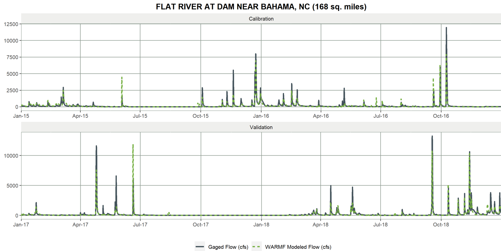
Figure G-35. Comparison of Observed and Simulated Stream Flows at Flat River at Dam near Bahama, NC (168 square miles)
