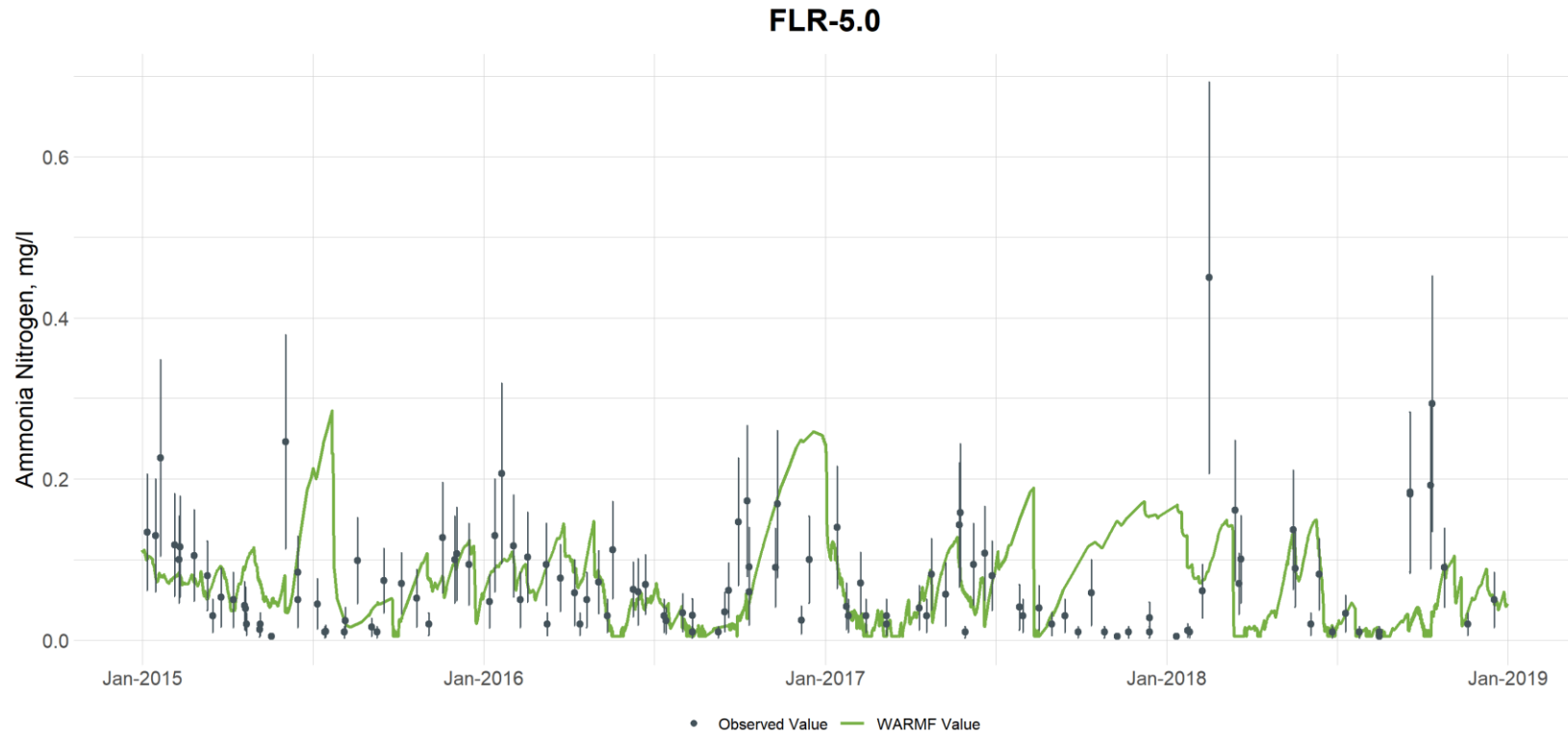
Figure G-45. Comparison of Observed and Simulated Ammonia Concentrations at Flat River at Station FLR-5 (downstream of Lake Michie) (vertical bars are used to illustrate the uncertainty with laboratory analyses and are based on the 95 th percentile confidence interval calculated from the UNRBA data set for each parameter)
