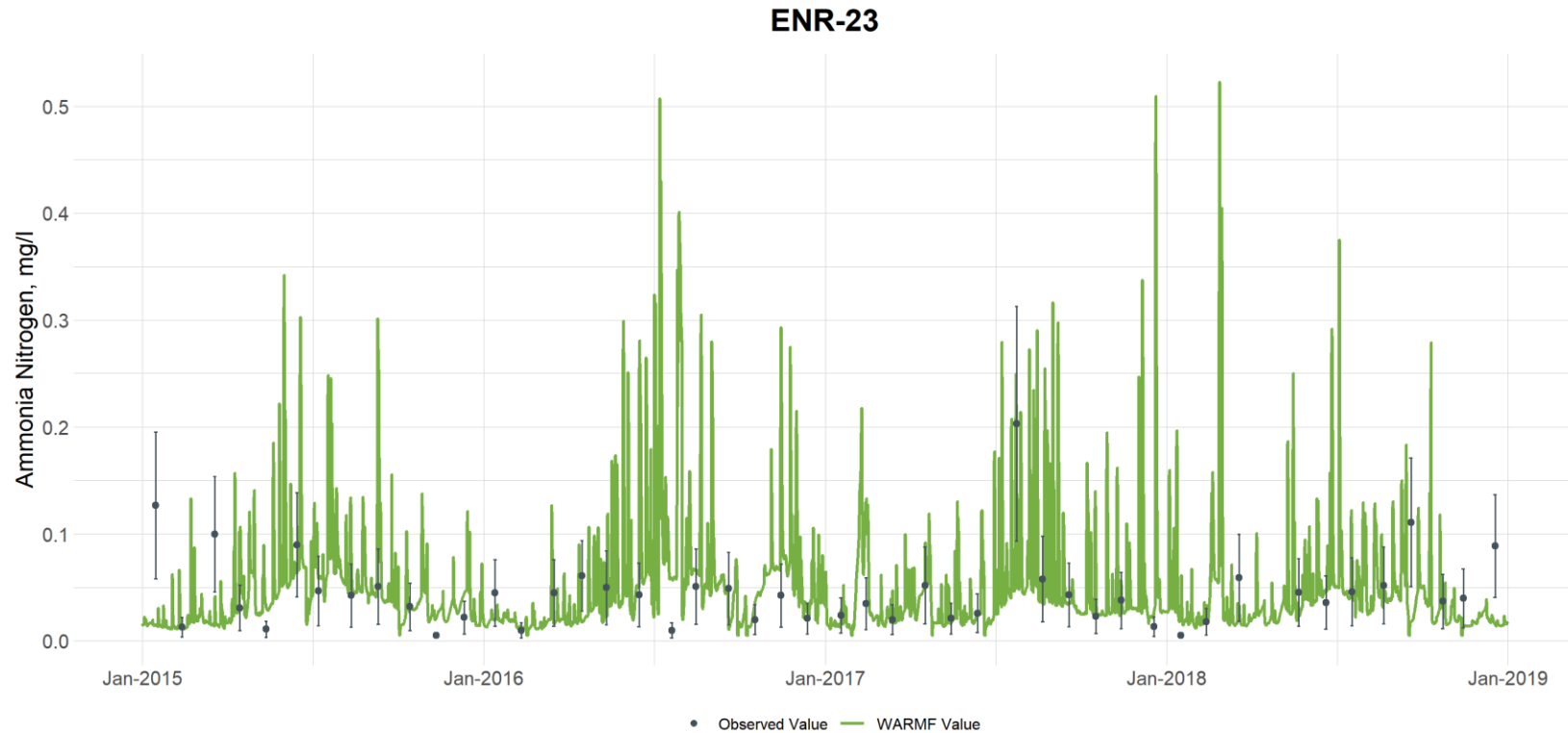
Figure G-17. Comparison of Observed and Simulated Ammonia Concentrations at Eno River at Station ENR-23 (vertical bars are used to illustrate the uncertainty with laboratory analyses and are based on the 95th percentile confidence interval calculated from the UNRBA data set for each parameter)
