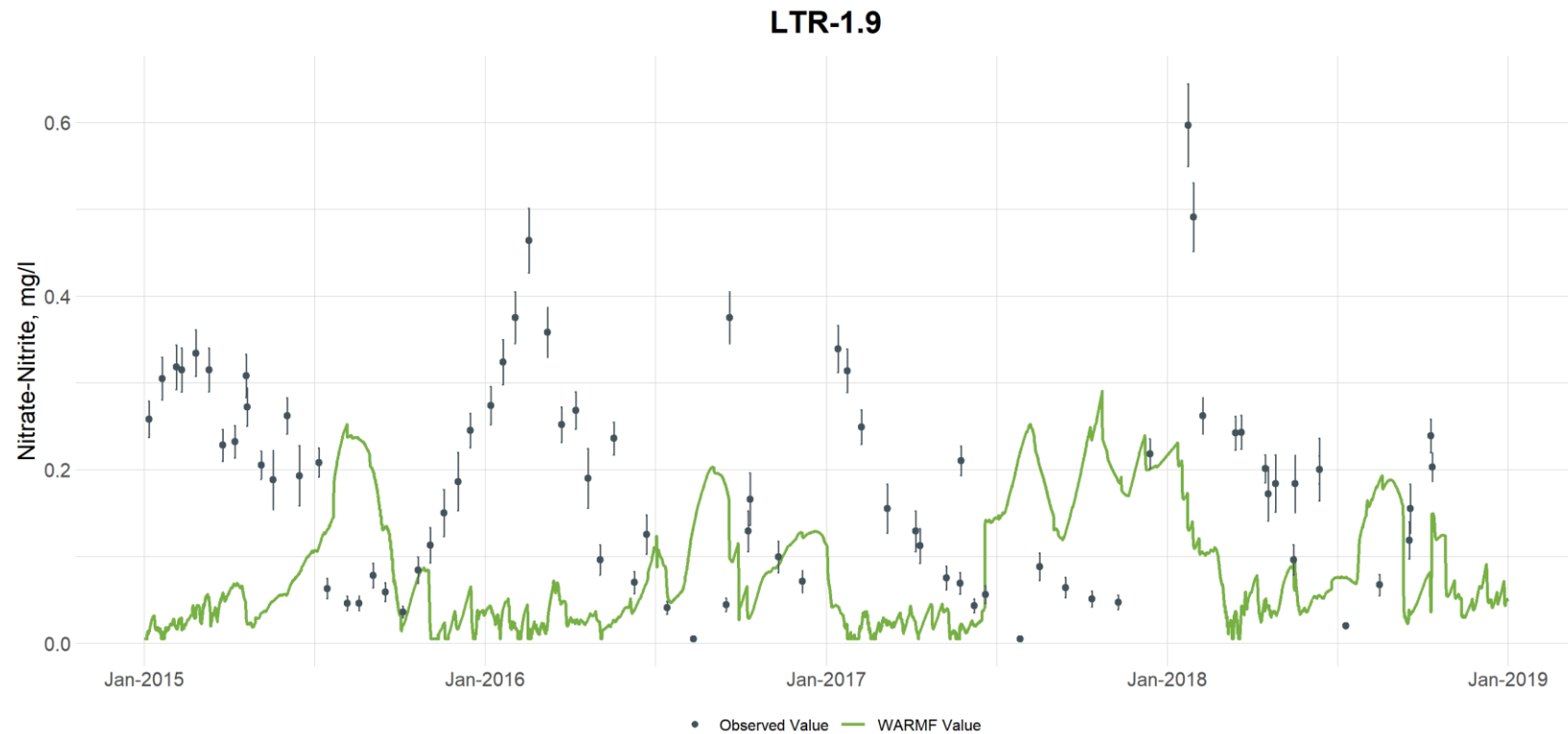
Figure G-76. Comparison of Observed and Simulated Nitrate-Nitrite Concentrations at Little River at Station LTR-1.9 (downstream of Little River Reservoir) (vertical bars are used to illustrate the uncertainty with laboratory analyses and are based on the 95th percentile confidence interval calculated from the UNRBA data set for each parameter)
