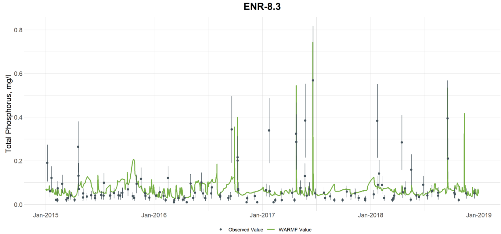
Figure G-30. Comparison of Observed and Simulated Total Phosphorus Concentrations at Eno River at Station ENR-8.3 (vertical bars are used to illustrate the uncertainty with laboratory analyses and are based on the 95th percentile confidence interval calculated from the UNRBA data set for each parameter)
