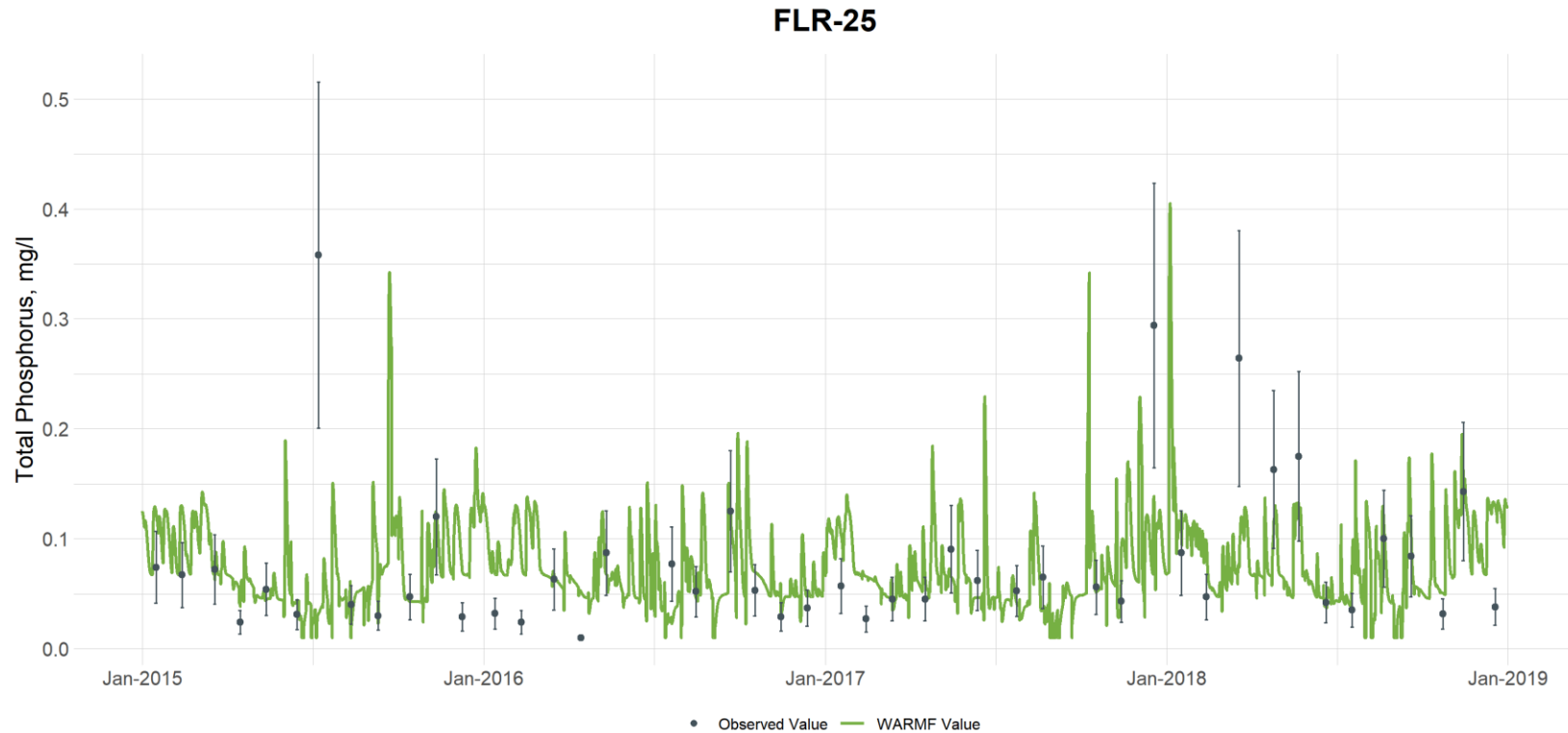
Figure G-42. Comparison of Observed and Simulated Total Phosphorus Concentrations at Flat River at Station FLR-25 (vertical bars are used to illustrate the uncertainty with laboratory analyses and are based on the 95 th percentile confidence interval calculated from the UNRBA data set for each parameter)
