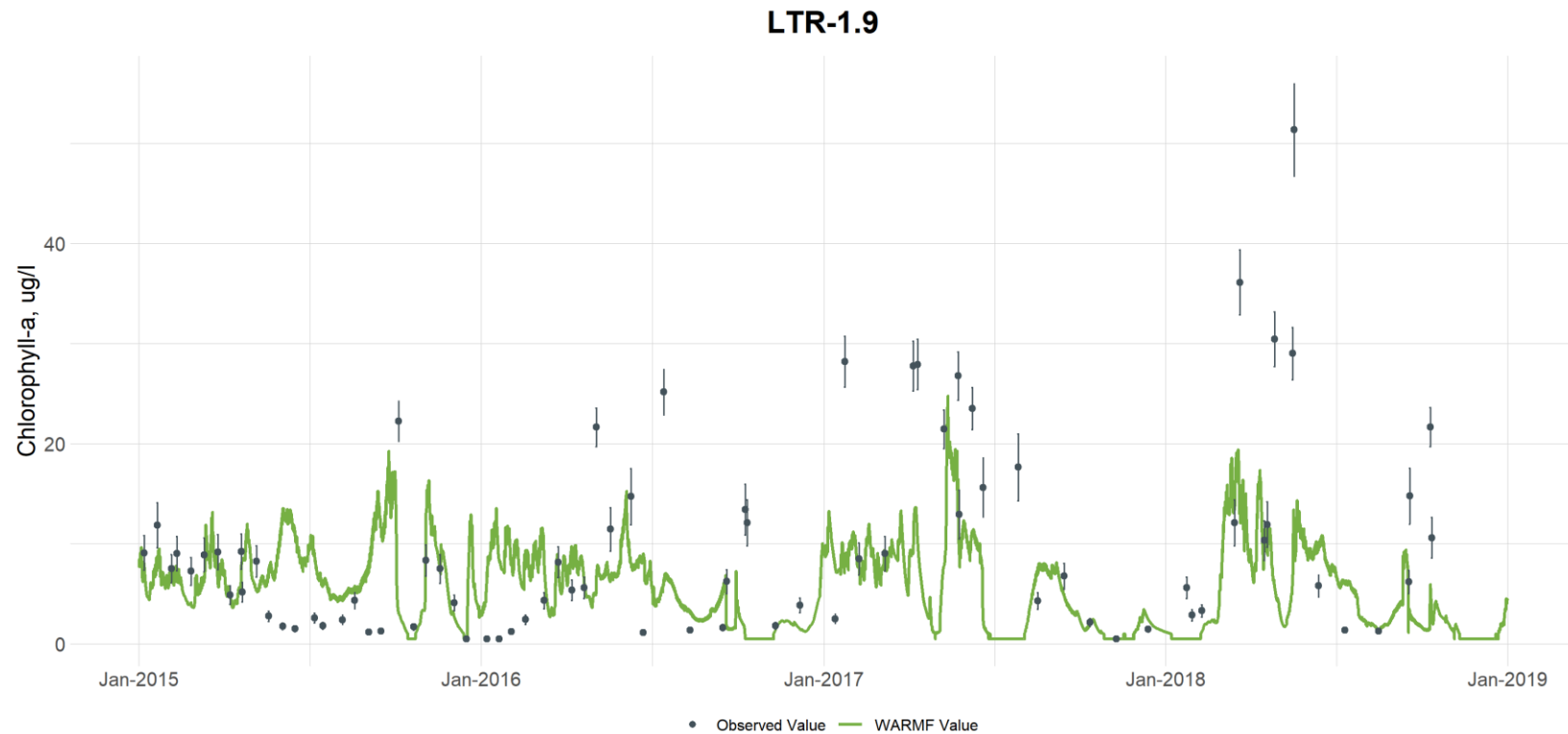
Figure G-83. Comparison of Observed and Simulated Chlorophyll-a Concentrations at Little River at Station LTR-1.9 (downstream of Little River Reservoir) (vertical bars are used to illustrate the uncertainty with laboratory analyses and are based on the 95th percentile confidence interval calculated from the UNRBA data set for each parameter)
