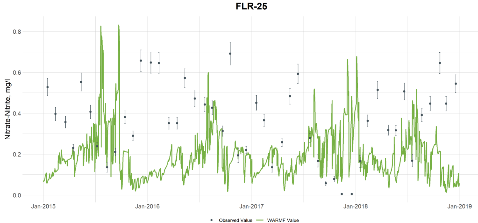
Figure G-38. Comparison of Observed and Simulated Nitrate-Nitrite Concentrations at Flat River at Station FLR-25 (vertical bars are used to illustrate the uncertainty with laboratory analyses and are based on the 95 th percentile confidence interval calculated from the UNRBA data set for each parameter)
