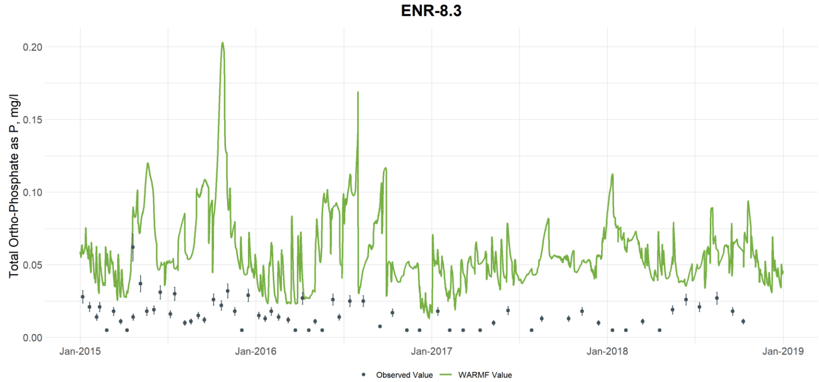
Figure G-31. Comparison of Observed and Simulated Total Ortho-Phosphate Concentrations at Eno River at Station ENR-8.3 (vertical bars are used to illustrate the uncertainty with laboratory analyses and are based on the 95 th percentile confidence interval calculated from the UNRBA data set for each parameter)
