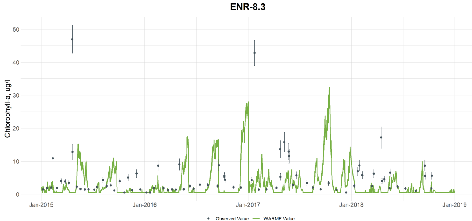
Figure G-33. Comparison of Observed and Simulated Chlorophyll-a Concentrations at Eno River at Station ENR-8.3 (vertical bars are used to illustrate the uncertainty with laboratory analyses and are based on the 95 th percentile confidence interval calculated from the UNRBA data set for each parameter)
