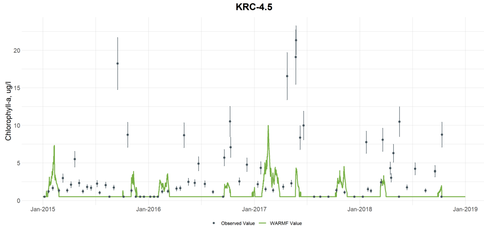
Figure G-64. Comparison of Observed and Simulated Chlorophyll-a Concentrations at Knap of Reeds Creek at Station KRC-4.5 (vertical bars are used to illustrate the uncertainty with laboratory analyses and are based on the 95th percentile confidence interval calculated from the UNRBA data set for each parameter)
