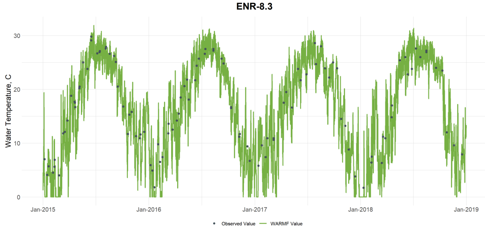
Figure G-24. Comparison of Observed and Simulated Stream Temperatures at Eno River at Station ENR-8.3
