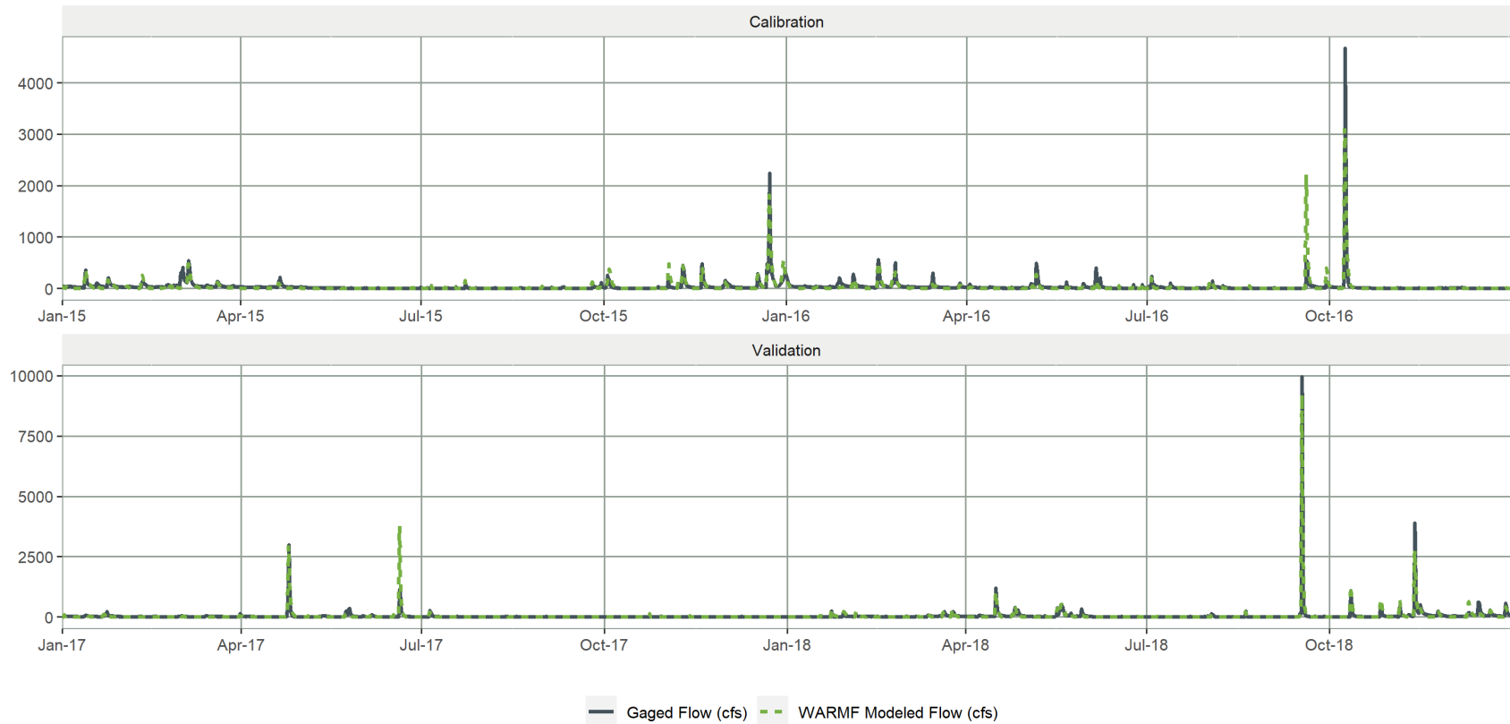
Figure G-54. Comparison of Observed and Simulated Stream Flows at Knap of Reeds Creek near Butner, NC (43 square miles)
