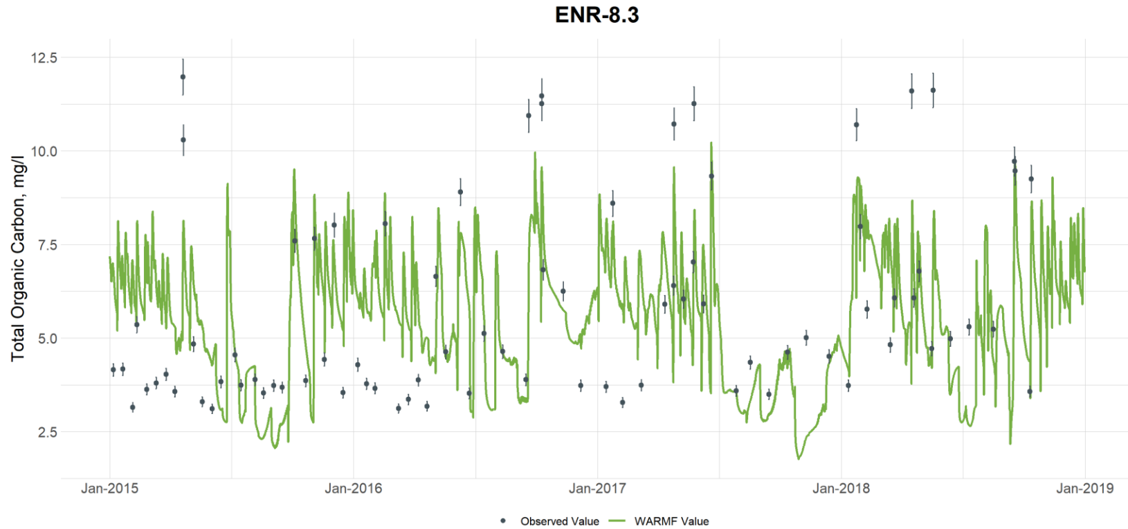
Figure G-29. Comparison of Observed and Simulated Total Organic Carbon Concentrations at Eno River at Station ENR-8.3 (vertical bars are used to illustrate the uncertainty with laboratory analyses and are based on the 95th percentile confidence interval calculated from the UNRBA data set for each parameter)
