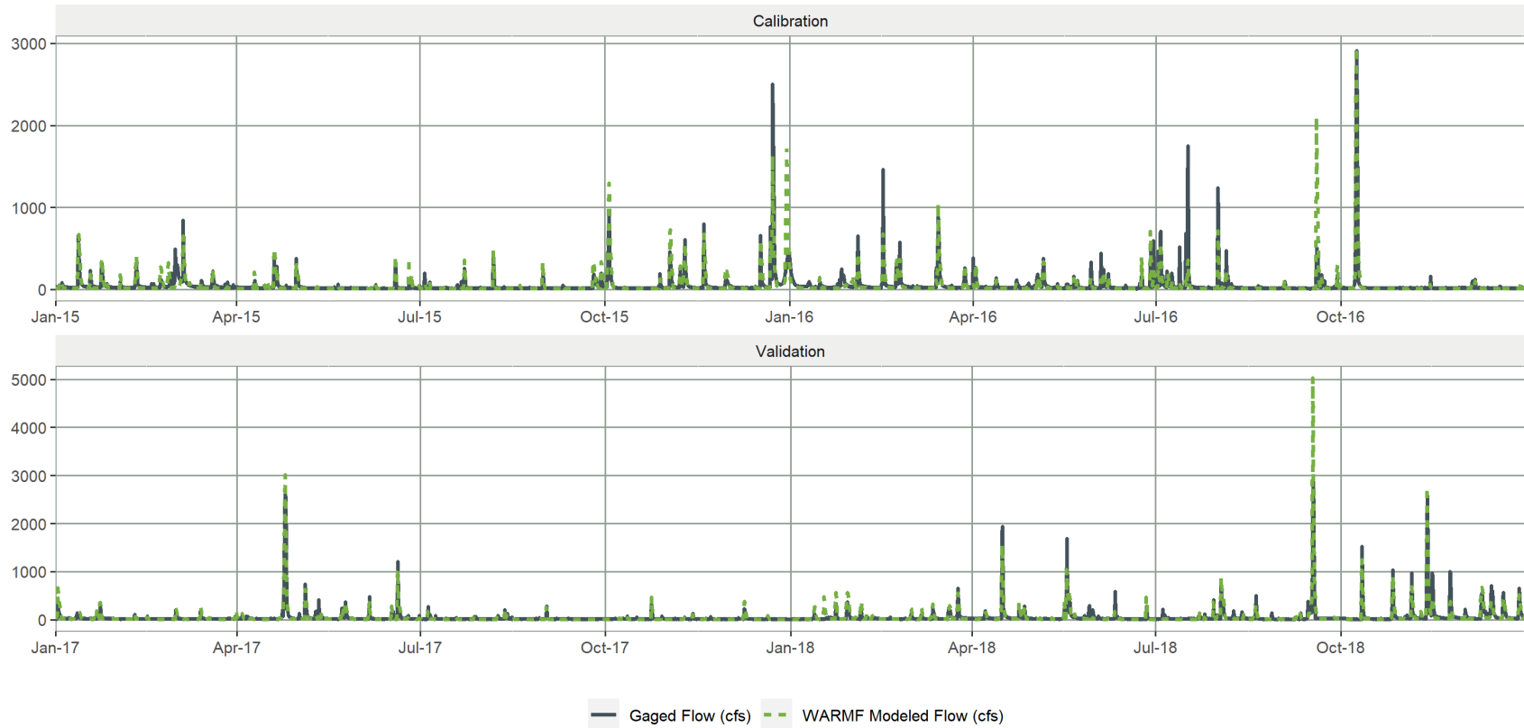
Figure G-3. Comparison of Observed and Simulated Stream Flows at Ellerbe Creek near Gorman, NC (21.9 square miles)
