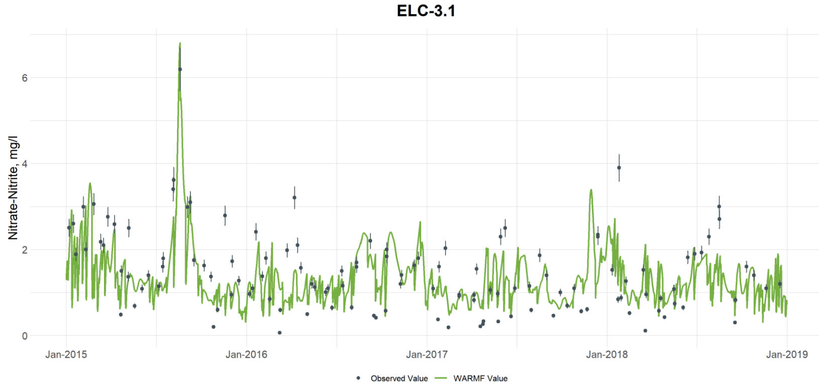
Figure G-6. Comparison of Observed and Simulated Nitrate-Nitrite Concentrations at Ellerbe Creek at Station ELC-3.1 (vertical bars are used to illustrate the uncertainty with laboratory analyses and are based on the 95th percentile confidence interval calculated from the UNRBA data set for each parameter)
