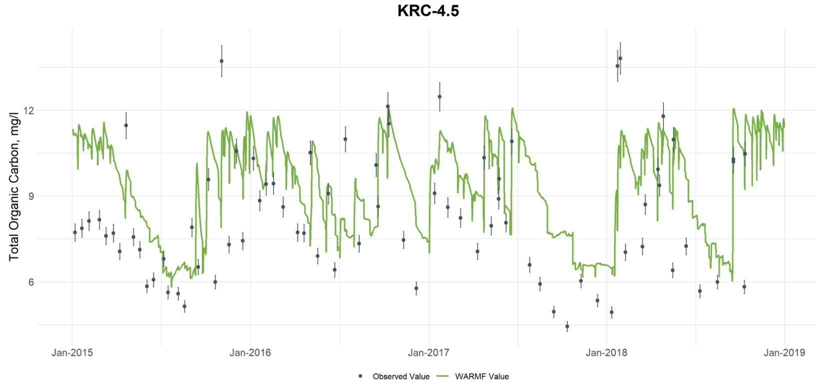
Figure G-60. Comparison of Observed and Simulated Total Organic Carbon Concentrations at Knap of Reeds Creek at Station KRC-4.5 (vertical bars are used to illustrate the uncertainty with laboratory analyses and are based on the 95th percentile confidence interval calculated from the UNRBA data set for each parameter)
