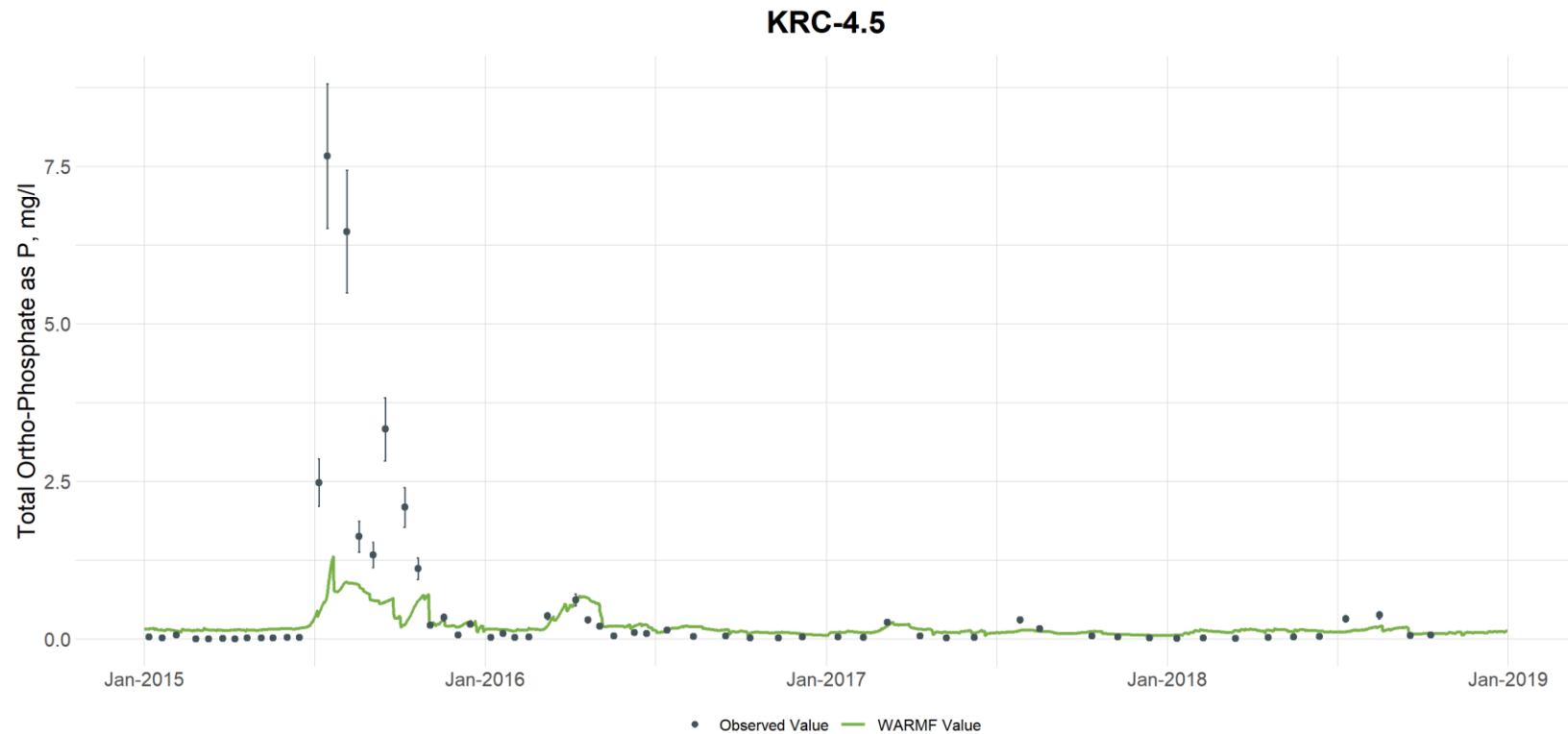
Figure G-62. Comparison of Observed and Simulated Total Ortho-Phosphate Concentrations at Knap of Reeds Creek at Station KRC-4.5 (vertical bars are used to illustrate the uncertainty with laboratory analyses and are based on the 95th percentile confidence interval calculated from the UNRBA data set for each parameter)
