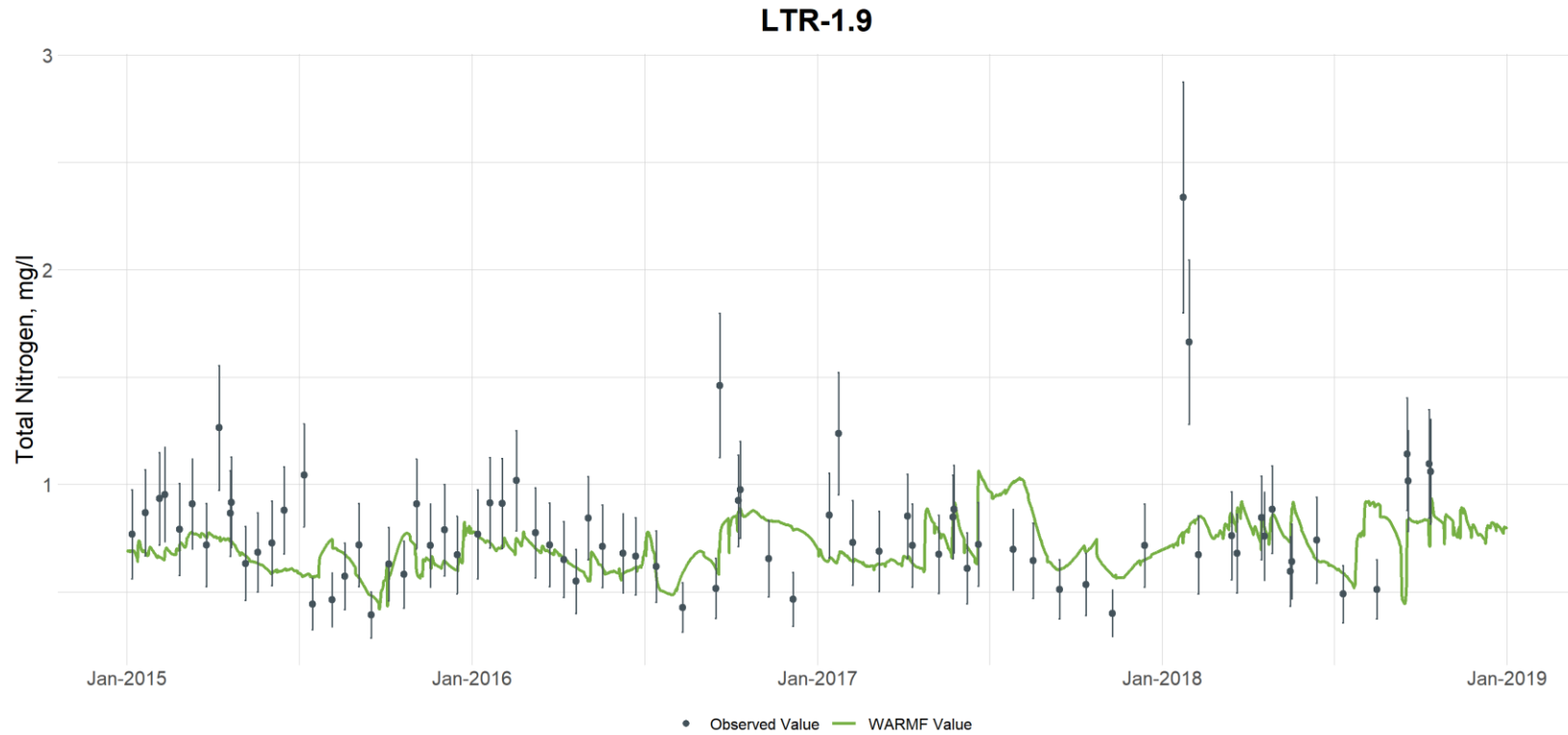
Figure G-78. Comparison of Observed and Simulated Total Nitrogen Concentrations at Little River at Station LTR-1.9 (downstream of Little River Reservoir) (vertical bars are used to illustrate the uncertainty with laboratory analyses and are based on the 95th percentile confidence interval calculated from the UNRBA data set for each parameter)
