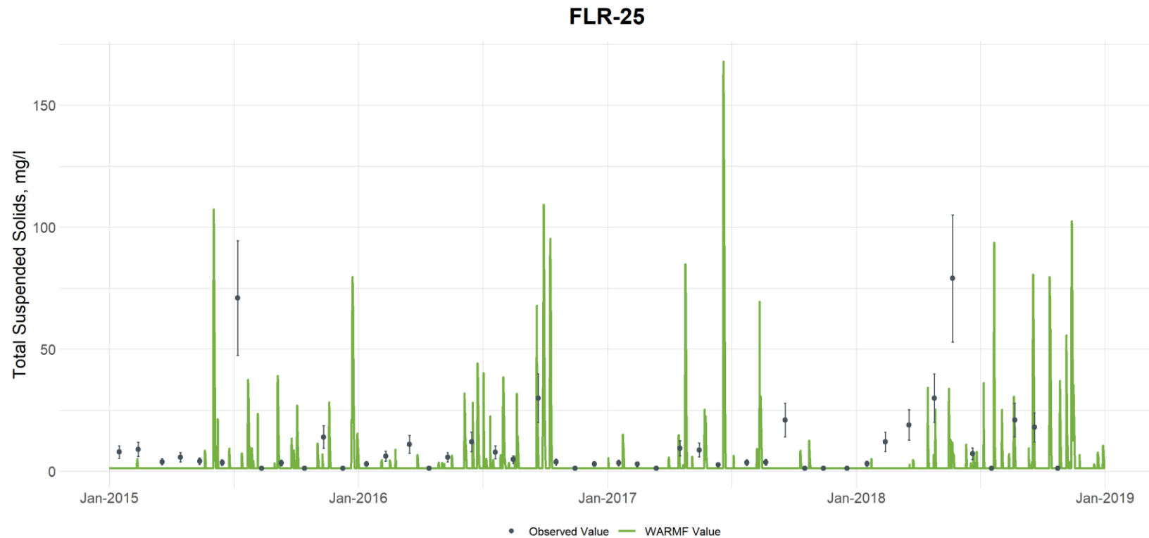
Figure G-43. Comparison of Observed and Simulated Total Suspended Solids (silt+clay) Concentrations at Flat River at Station FLR-25 (vertical bars are used to illustrate the uncertainty with laboratory analyses and are based on the 95 th percentile confidence interval calculated from the UNRBA data set for each parameter)
