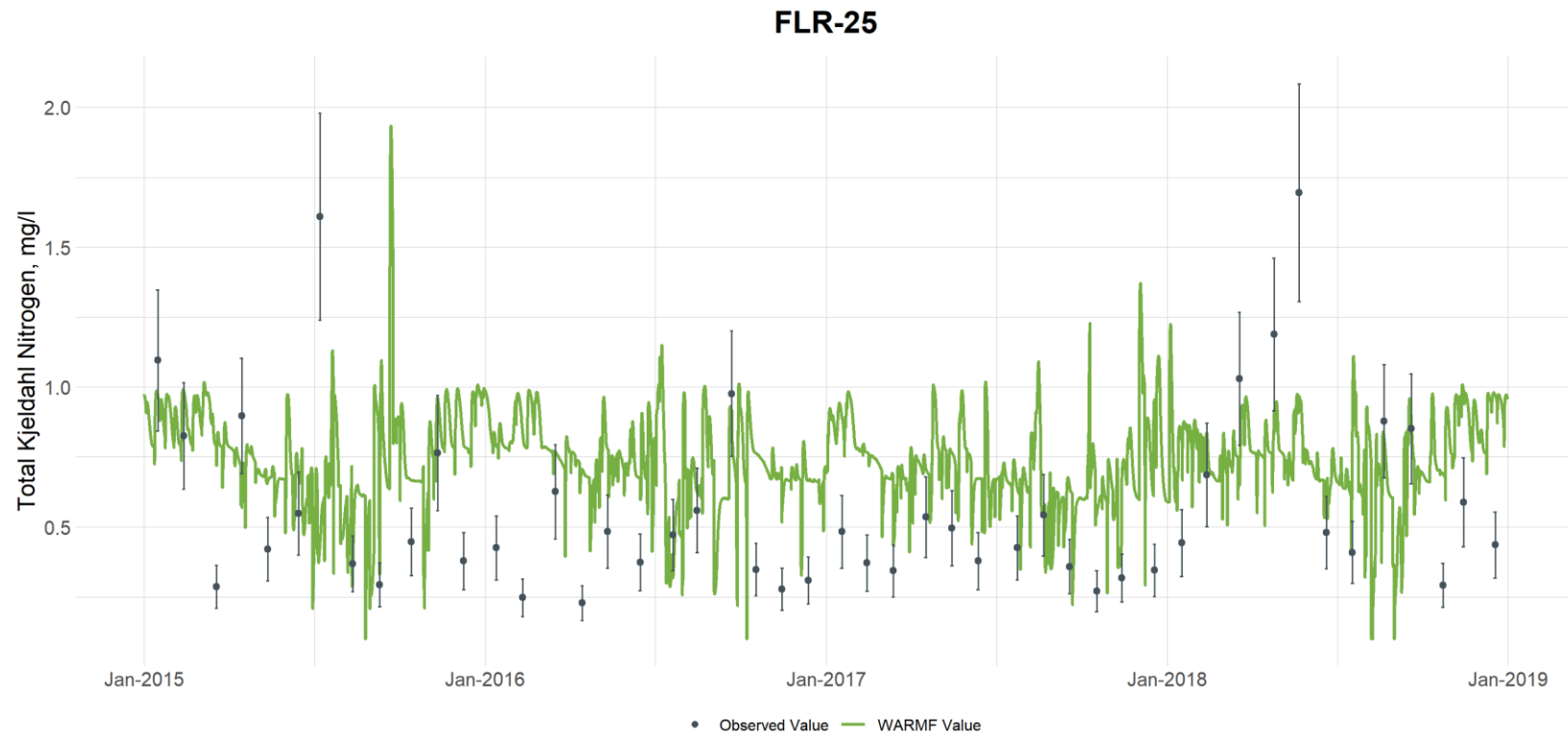
Figure G-39. Comparison of Observed and Simulated Total Kjeldahl Nitrogen Concentrations at Flat River at Station FLR-25 (vertical bars are used to illustrate the uncertainty with laboratory analyses and are based on the 95 th percentile confidence interval calculated from the UNRBA data set for each parameter)
