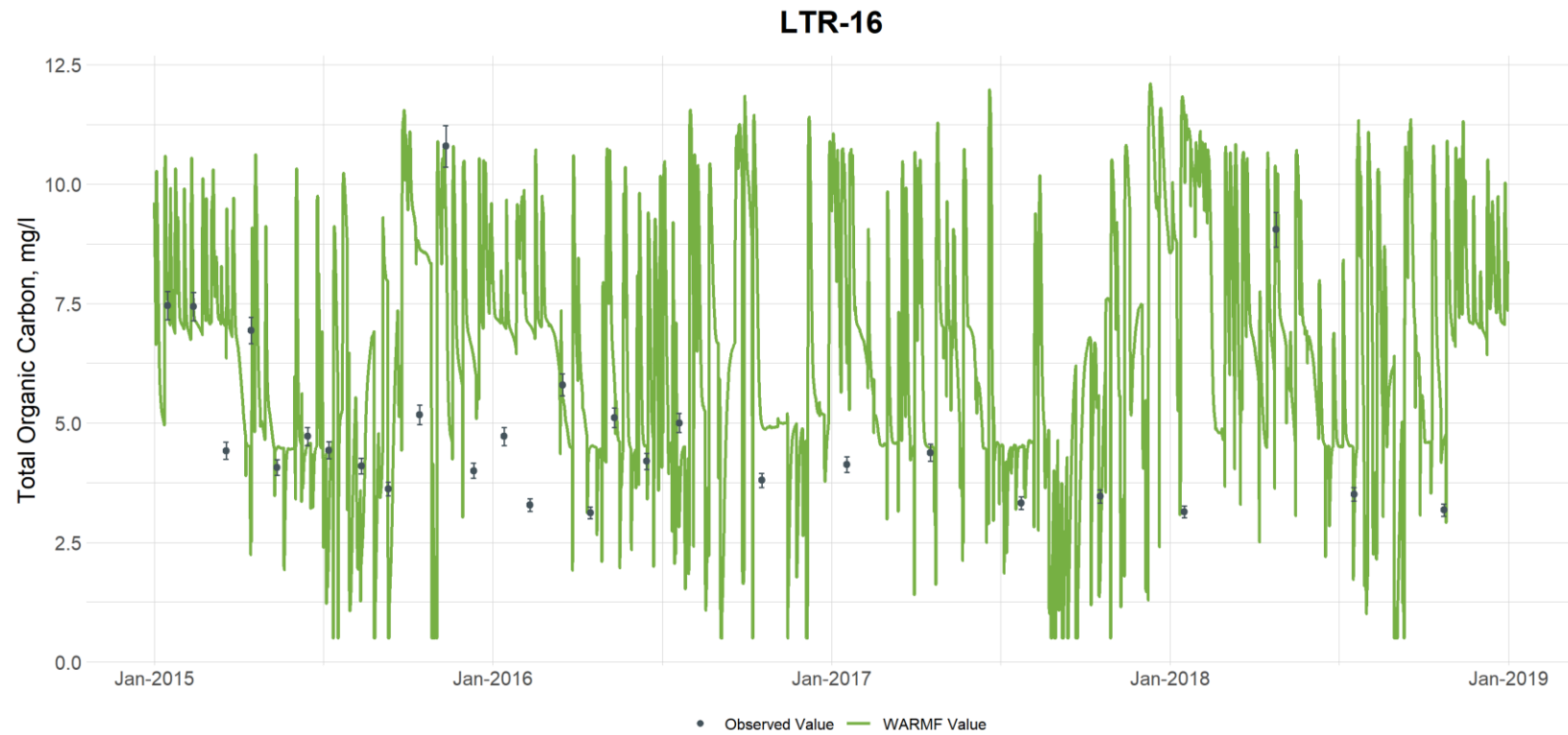
Figure G-71. Comparison of Observed and Simulated Total Organic Carbon Concentrations at Little River at Station LTR-16 (vertical bars are used to illustrate the uncertainty with laboratory analyses and are based on the 95th percentile confidence interval calculated from the UNRBA data set for each parameter)
