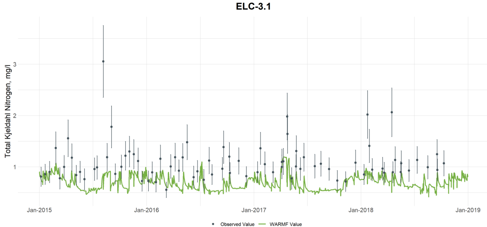
Figure G-7. Comparison of Observed and Simulated Total Kjeldahl Nitrogen Concentrations at Ellerbe Creek at Station ELC-3.1 (vertical bars are used to illustrate the uncertainty with laboratory analyses and are based on the 95th percentile confidence interval calculated from the UNRBA data set for each parameter)
