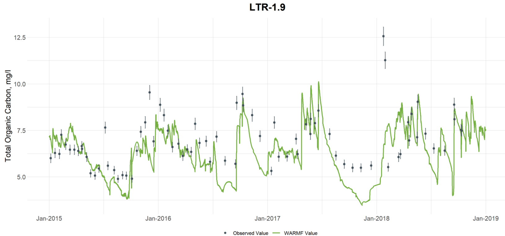
Figure G-79. Comparison of Observed and Simulated Total Organic Carbon Concentrations at Little River at Station LTR-1.9 (downstream of Little River Reservoir) (vertical bars are used to illustrate the uncertainty with laboratory analyses and are based on the 95th percentile confidence interval calculated from the UNRBA data set for each parameter)
