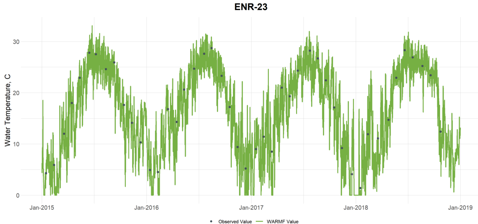
Figure G-16. Comparison of Observed and Simulated Stream Temperatures at Eno River at Station ENR-23
