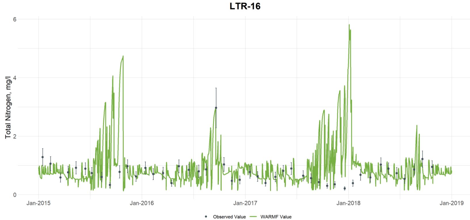
Figure G-70. Comparison of Observed and Simulated Total Nitrogen Concentrations at Little River at Station LTR-16 (vertical bars are used to illustrate the uncertainty with laboratory analyses and are based on the 95th percentile confidence interval calculated from the UNRBA data set for each parameter)
