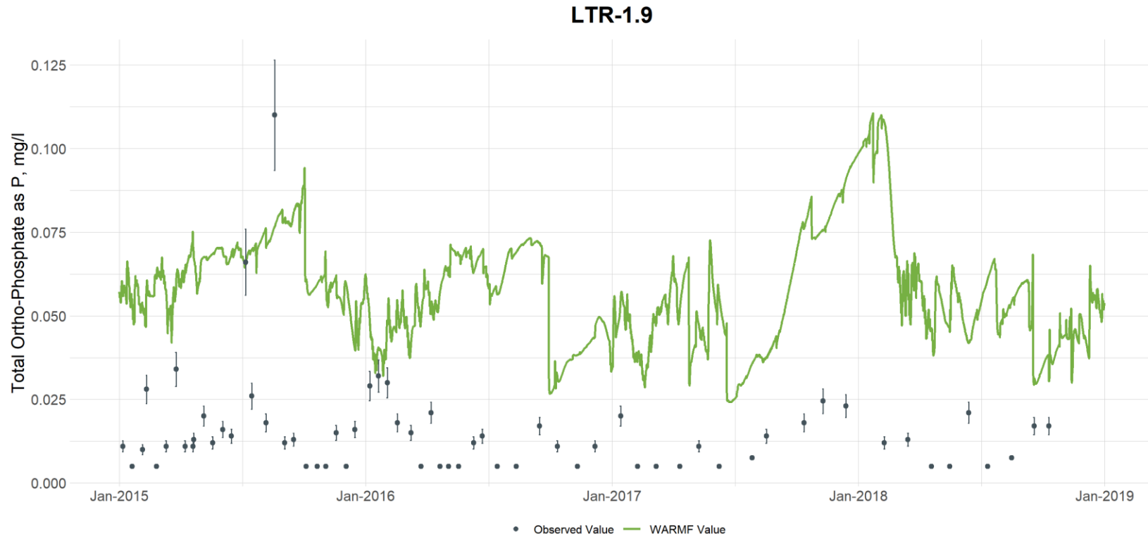
Figure G-81. Comparison of Observed and Simulated Total Ortho-Phosphate Concentrations at Little River at Station LTR-1.9 (downstream of Little River Reservoir) (vertical bars are used to illustrate the uncertainty with laboratory analyses and are based on the 95th percentile confidence interval calculated from the UNRBA data set for each parameter)
