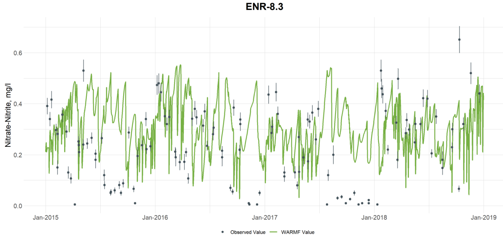
Figure G-26. Comparison of Observed and Simulated Nitrate-Nitrite Concentrations at Eno River at Station ENR-8.3 (vertical bars are used to illustrate the uncertainty with laboratory analyses and are based on the 95th percentile confidence interval calculated from the UNRBA data set for each parameter)
