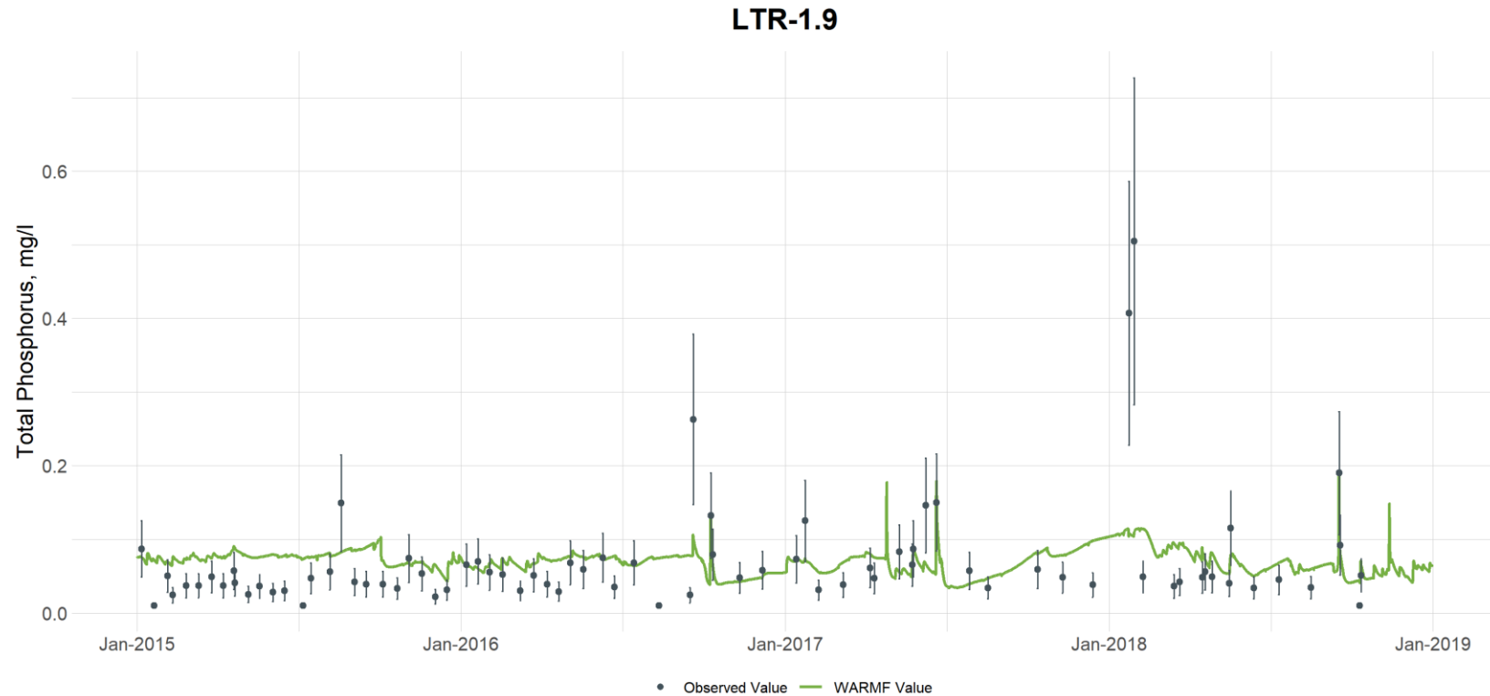
Figure G-80. Comparison of Observed and Simulated Total Phosphorus Concentrations at Little River at Station LTR-1.9 (downstream of Little River Reservoir) (vertical bars are used to illustrate the uncertainty with laboratory analyses and are based on the 95th percentile confidence interval calculated from the UNRBA data set for each parameter)
