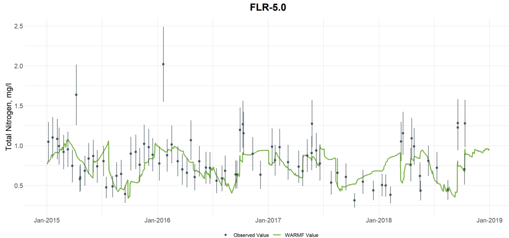
Figure G-48. Comparison of Observed and Simulated Total Nitrogen Concentrations at Flat River at Station FLR-5 (downstream of Lake Michie) (vertical bars are used to illustrate the uncertainty with laboratory analyses and are based on the 95 th percentile confidence interval calculated from the UNRBA data set for each parameter)
