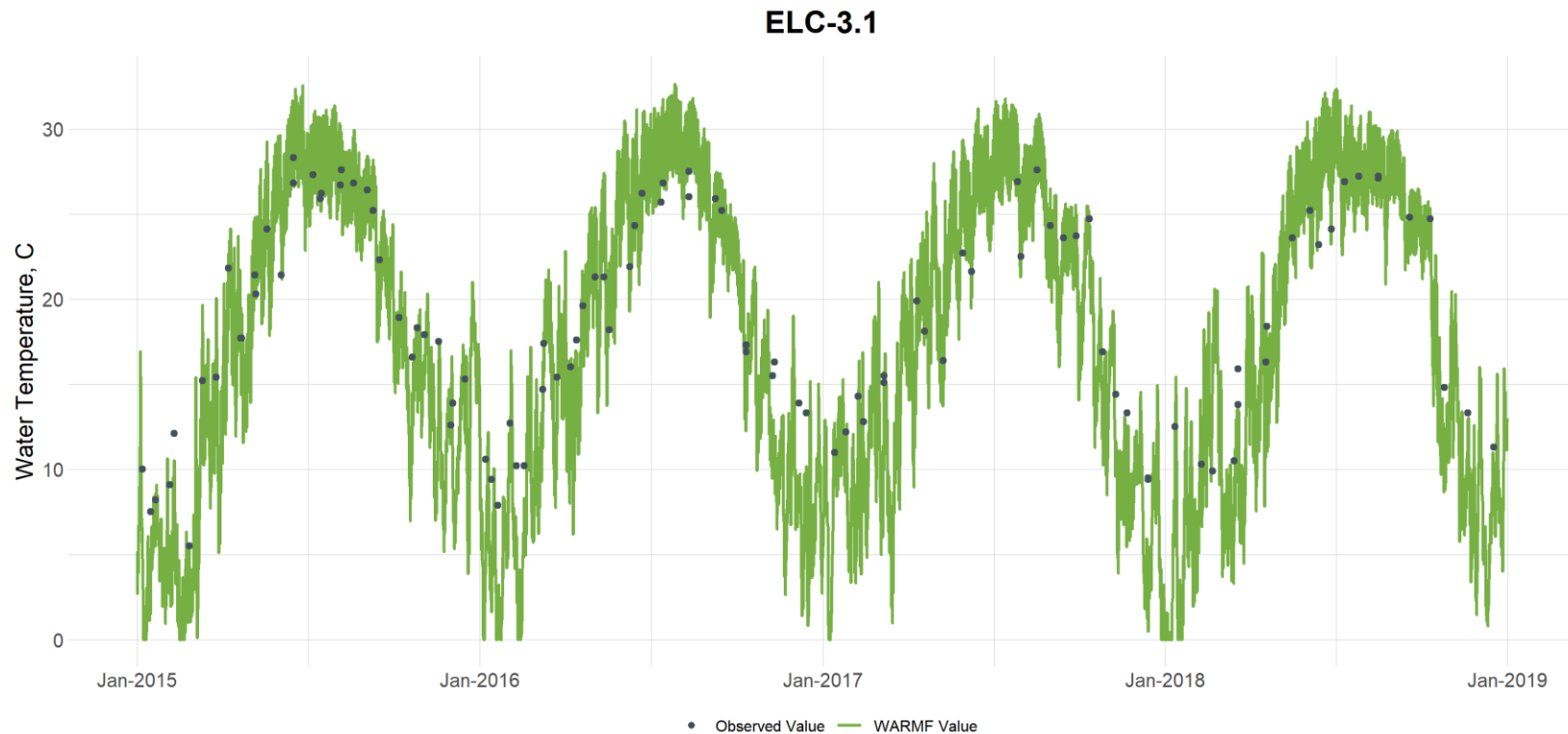
Figure G-4. Comparison of Observed and Simulated Stream Temperatures at Ellerbe Creek at Station ELC-3.1
