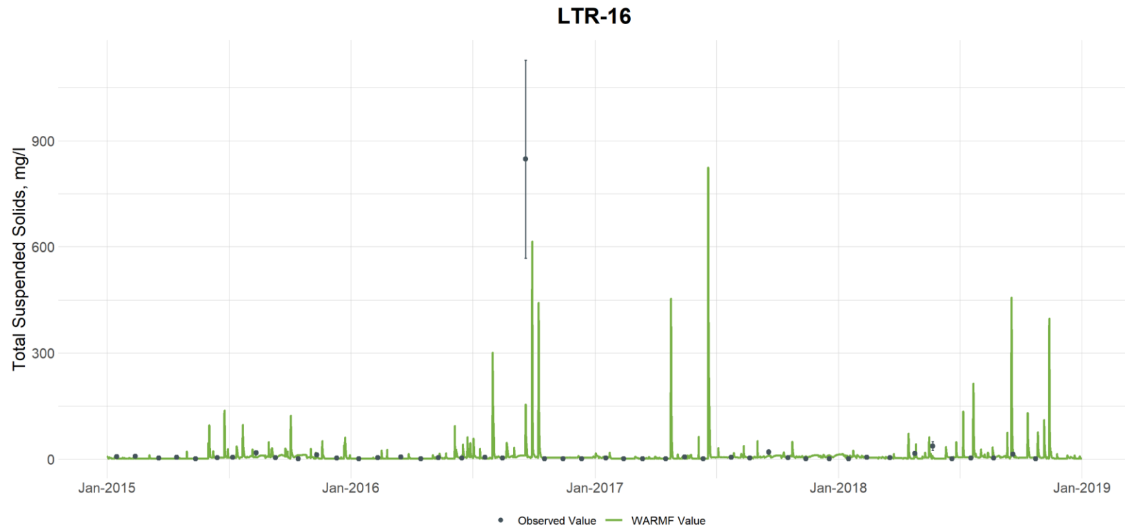
Figure G-73. Comparison of Observed and Simulated Total Suspended Solids (silt+clay) Concentrations at Little River at Station LTR-16 (vertical bars are used to illustrate the uncertainty with laboratory analyses and are based on the 95th percentile confidence interval calculated from the UNRBA data set for each parameter)
