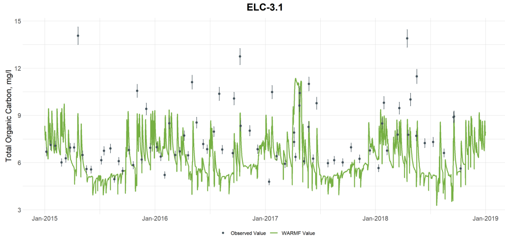
Figure G-9. Comparison of Observed and Simulated Total Organic Carbon Concentrations at Ellerbe Creek at Station ELC-3.1 (vertical bars are used to illustrate the uncertainty with laboratory analyses and are based on the 95th percentile confidence interval calculated from the UNRBA data set for each parameter)
