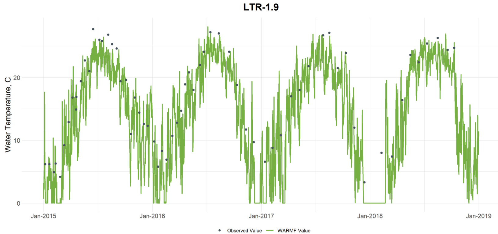
Figure G-74. Comparison of Observed and Simulated Stream Temperatures at Little River at Station LTR-1.9 (downstream of Little River Reservoir)
