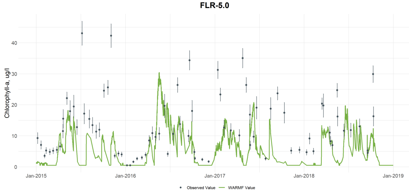
Figure G-53. Comparison of Observed and Simulated Chlorophyll-a Concentrations at Flat River at Station FLR-5 (downstream of Lake Michie) (vertical bars are used to illustrate the uncertainty with laboratory analyses and are based on the 95th percentile confidence interval calculated from the UNRBA data set for each parameter)
