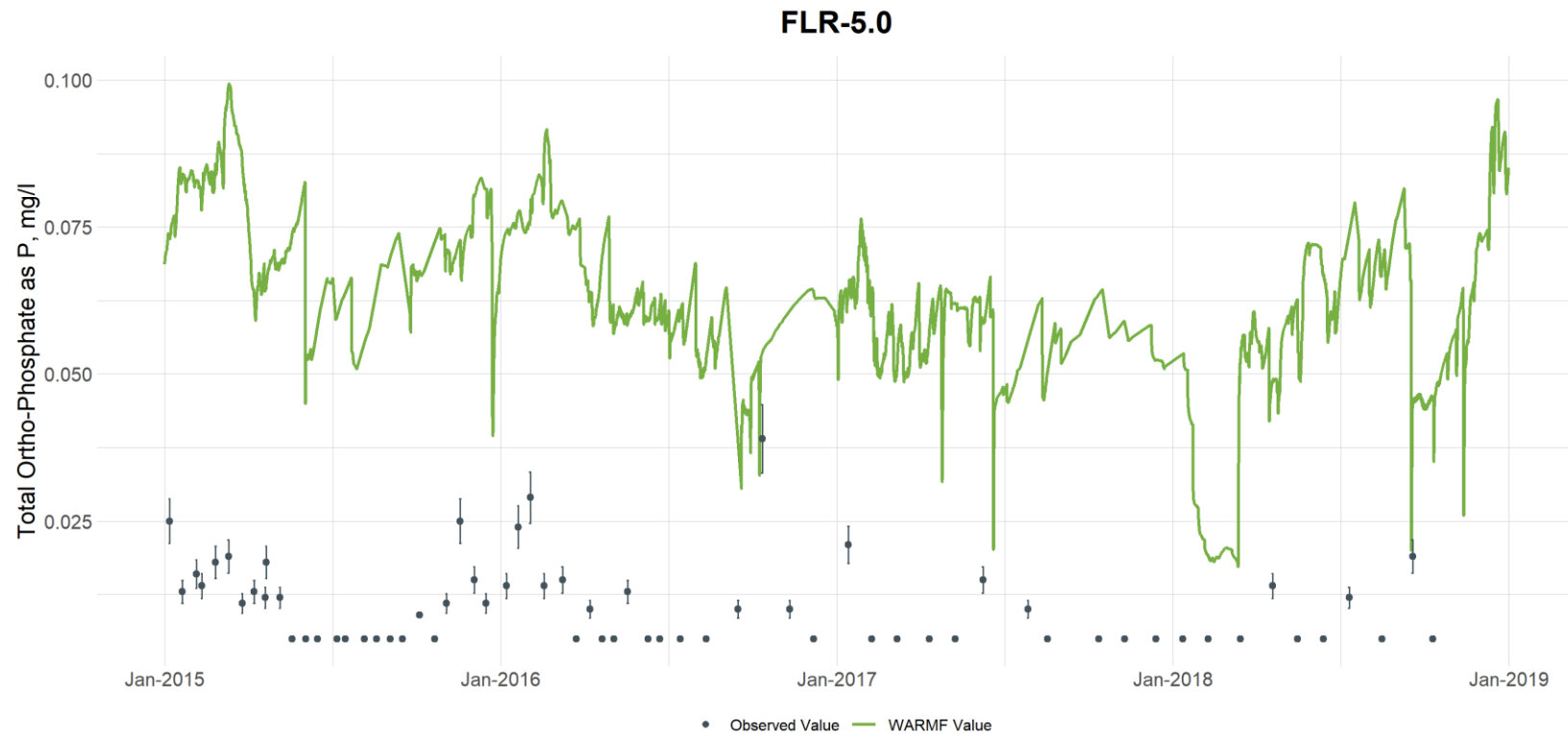
Figure G-51. Comparison of Observed and Simulated Total Ortho-Phosphate Concentrations at Flat River at Station FLR-5 (downstream of Lake Michie) (vertical bars are used to illustrate the uncertainty with laboratory analyses and are based on the 95th percentile confidence interval calculated from the UNRBA data set for each parameter)
