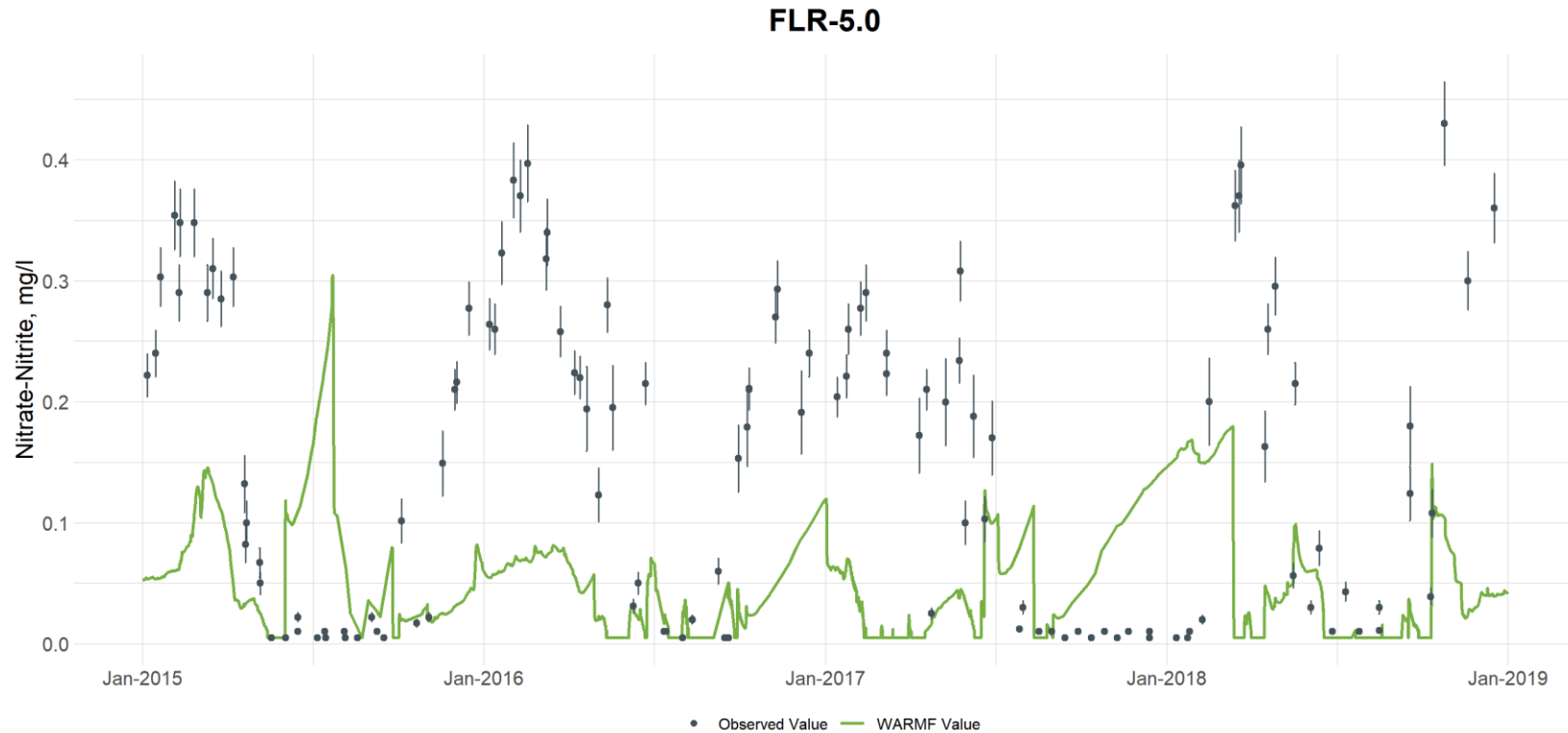
Figure G-46. Comparison of Observed and Simulated Nitrate-Nitrite Concentrations at Flat River at Station FLR-5 (downstream of Lake Michie) (vertical bars are used to illustrate the uncertainty with laboratory analyses and are based on the 95 th percentile confidence interval calculated from the UNRBA data set for each parameter)
