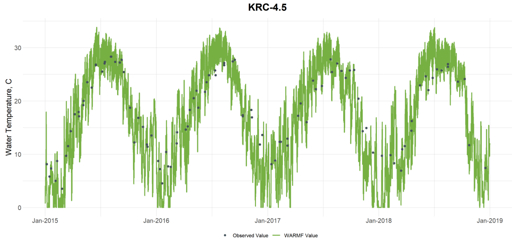
Figure G-55. Comparison of Observed and Simulated Stream Temperatures at Knap of Reeds Creek at Station KRC-4.5
