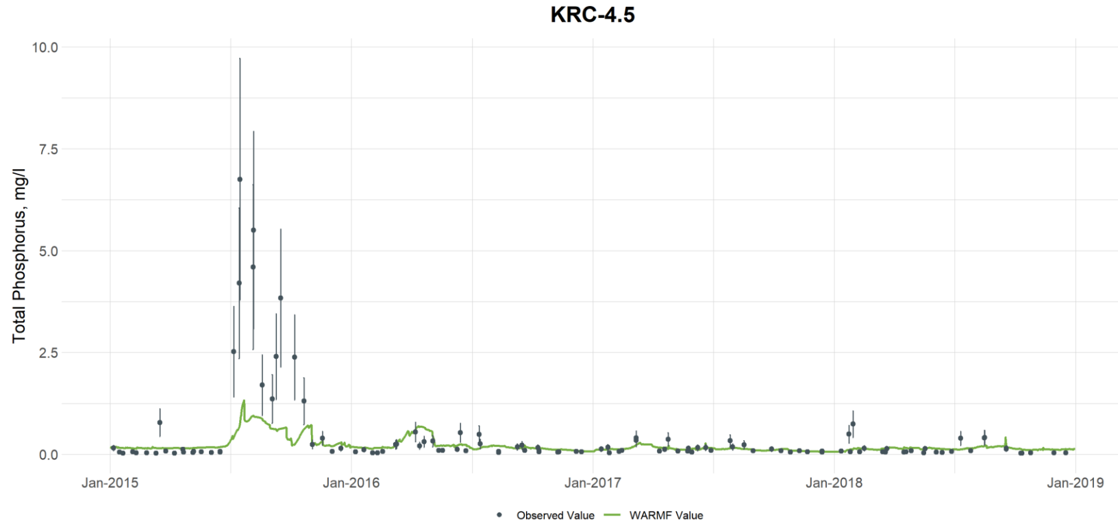
Figure G-61. Comparison of Observed and Simulated Total Phosphorus Concentrations at Knap of Reeds Creek at Station KRC-4.5 (vertical bars are used to illustrate the uncertainty with laboratory analyses and are based on the 95th percentile confidence interval calculated from the UNRBA data set for each parameter)
