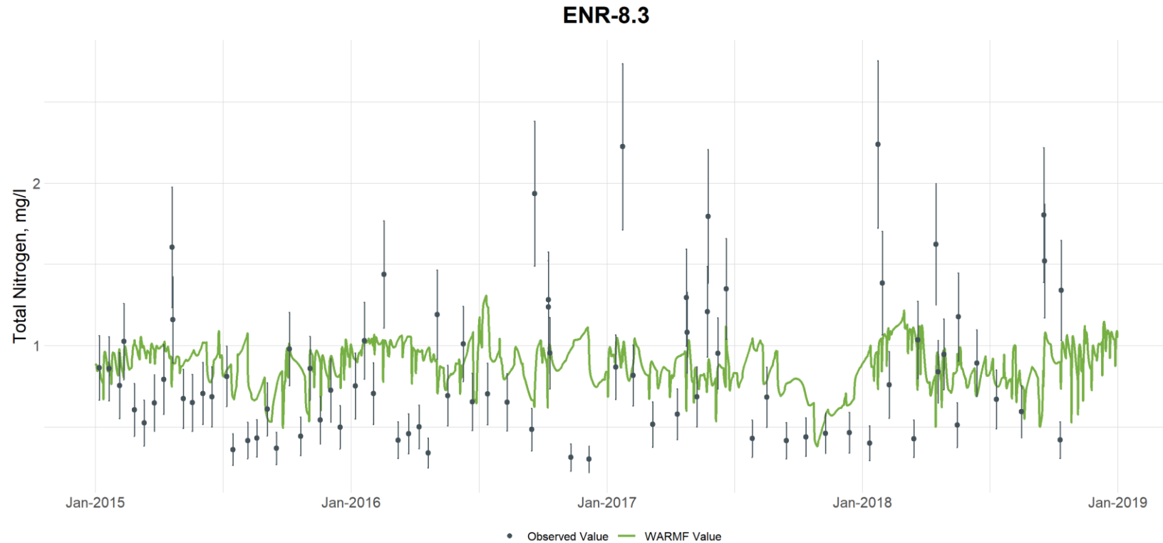
Figure G-28. Comparison of Observed and Simulated Total Nitrogen Concentrations at Eno River at Station ENR-8.3 (vertical bars are used to illustrate the uncertainty with laboratory analyses and are based on the 95th percentile confidence interval calculated from the UNRBA data set for each parameter)
