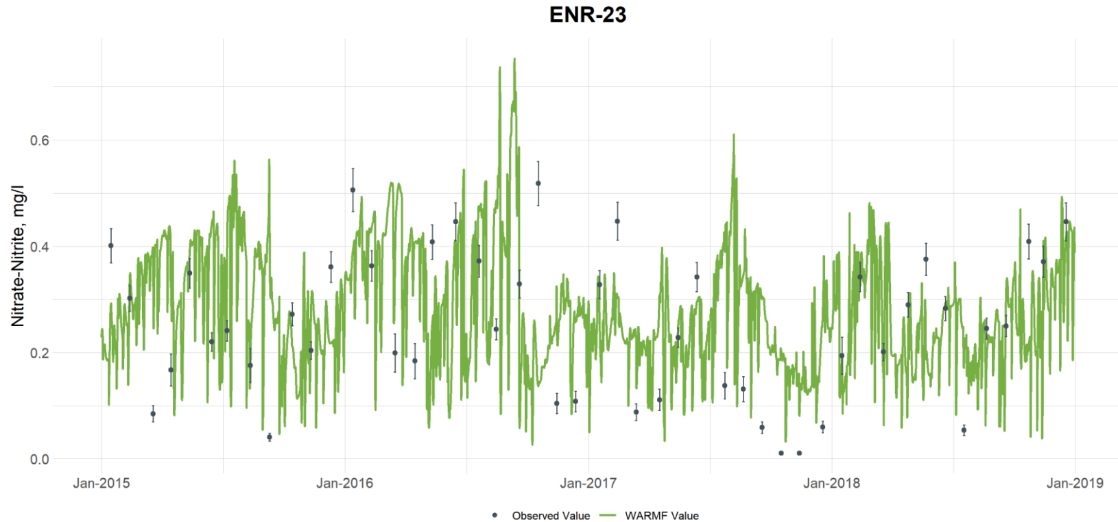
Figure G-18. Comparison of Observed and Simulated Nitrate-Nitrite Concentrations at Eno River at Station ENR-23 (vertical bars are used to illustrate the uncertainty with laboratory analyses and are based on the 95th percentile confidence interval calculated from the UNRBA data set for each parameter)
