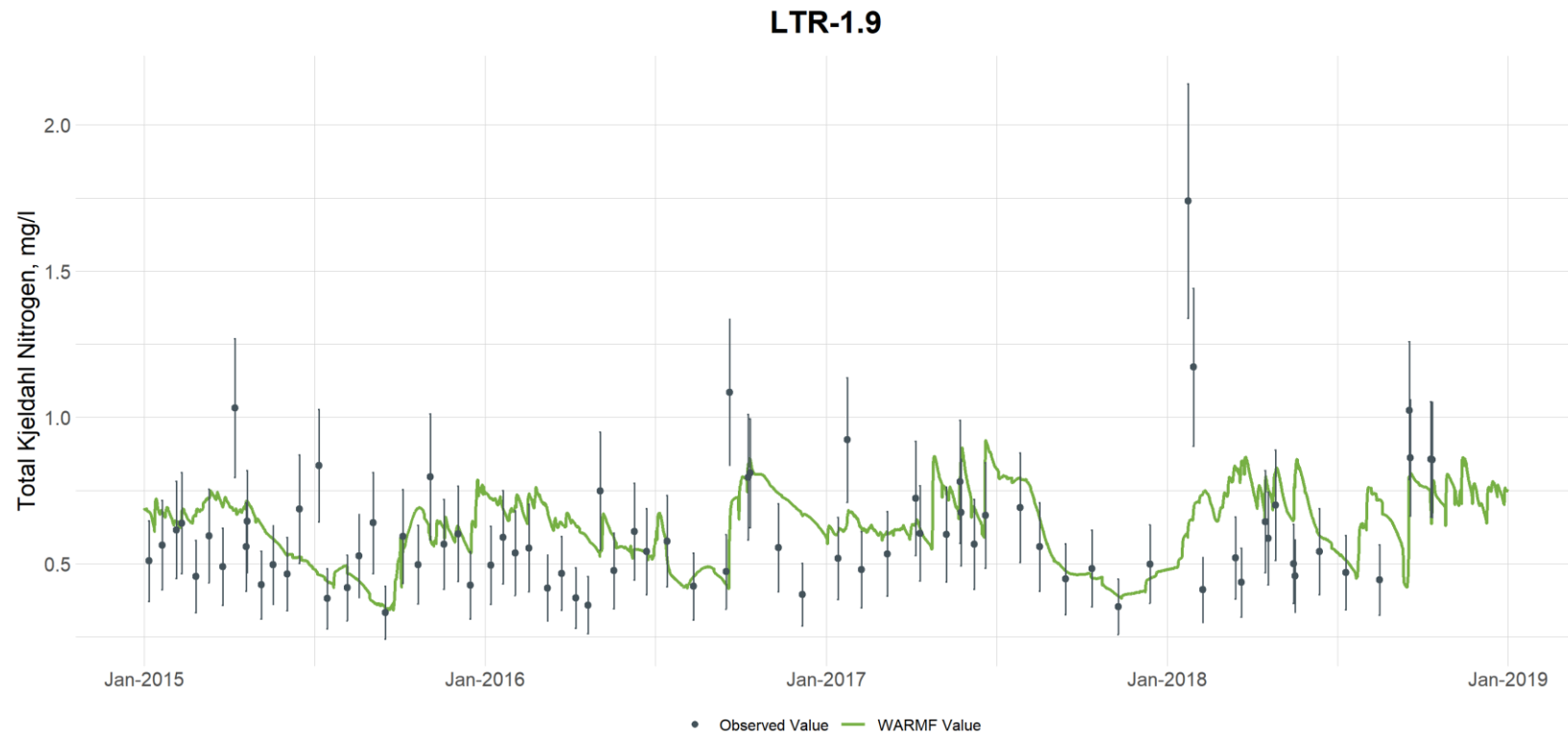
Figure G-77. Comparison of Observed and Simulated Total Kjeldahl Nitrogen Concentrations at Little River at Station LTR-1.9 (downstream of Little River Reservoir) (vertical bars are used to illustrate the uncertainty with laboratory analyses and are based on the 95th percentile confidence interval calculated from the UNRBA data set for each parameter)
