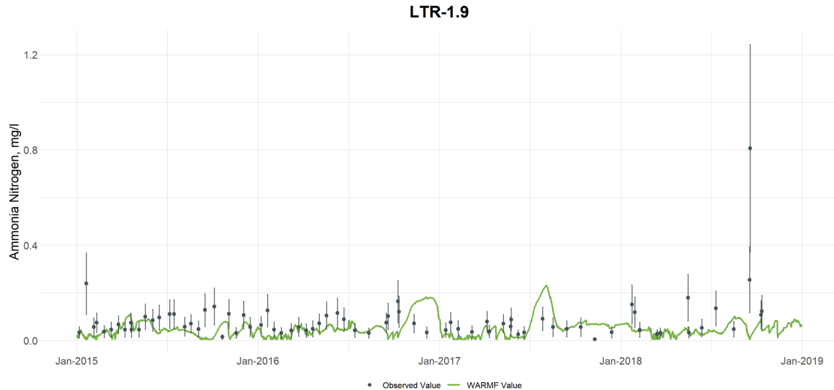
Figure G-75. Comparison of Observed and Simulated Ammonia Concentrations at Little River at Station LTR-1.9 (downstream of Little River Reservoir) (vertical bars are used to illustrate the uncertainty with laboratory analyses and are based on the 95th percentile confidence interval calculated from the UNRBA data set for each parameter)
