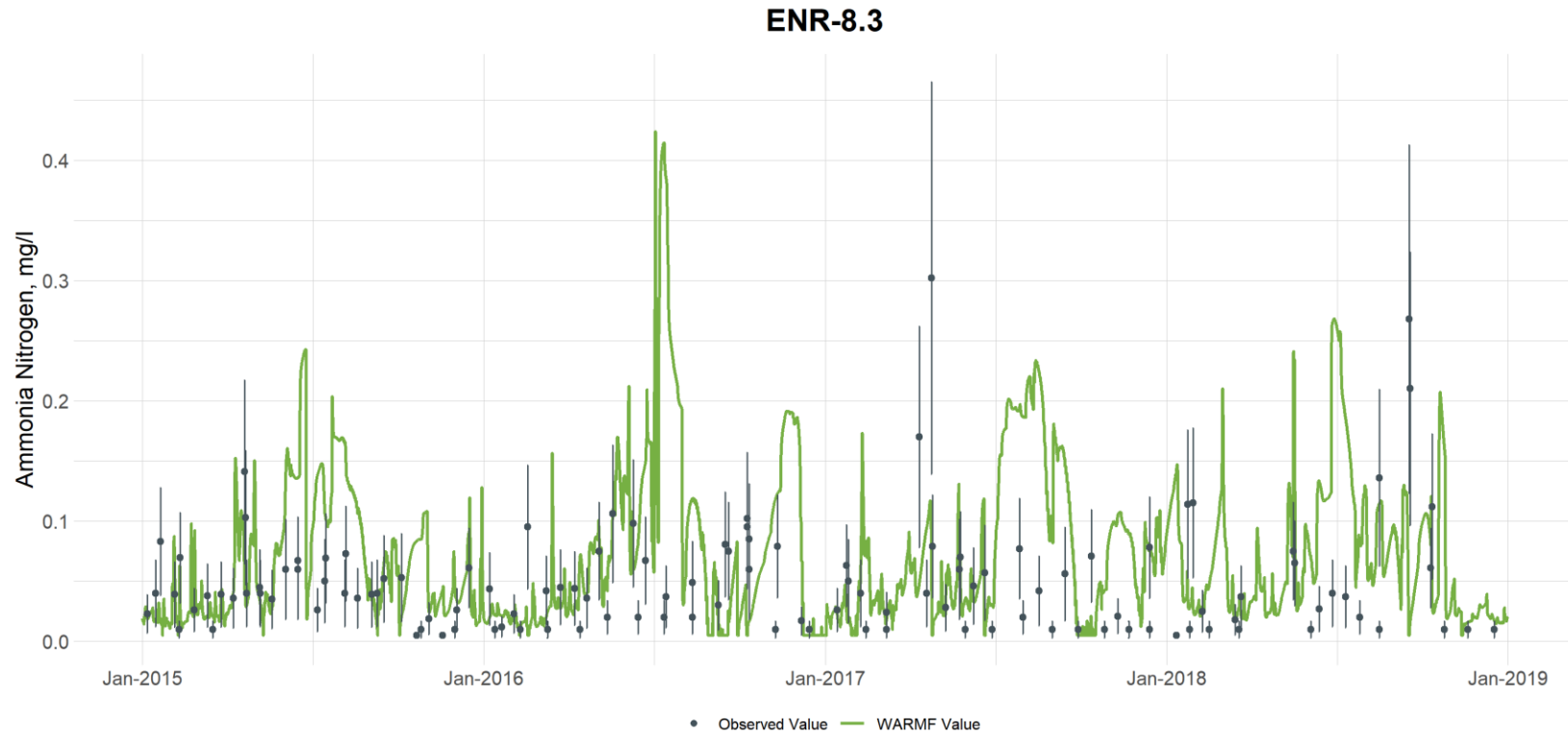
Figure G-25. Comparison of Observed and Simulated Ammonia Concentrations at Eno River at Station ENR-8.3 (vertical bars are used to illustrate the uncertainty with laboratory analyses and are based on the 95th percentile confidence interval calculated from the UNRBA data set for each parameter)
