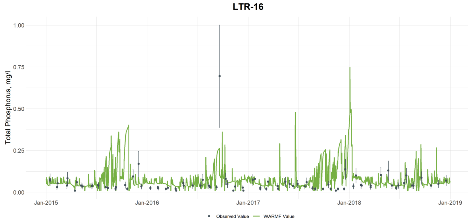
Figure G-72. Comparison of Observed and Simulated Total Phosphorus Concentrations at Little River at Station LTR-16 (vertical bars are used to illustrate the uncertainty with laboratory analyses and are based on the 95th percentile confidence interval calculated from the UNRBA data set for each parameter)
