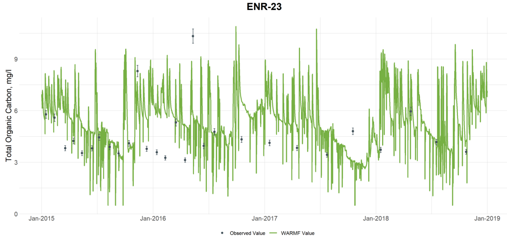
Figure G-21. Comparison of Observed and Simulated Total Organic Carbon Concentrations at Eno River at Station ENR-23 (vertical bars are used to illustrate the uncertainty with laboratory analyses and are based on the 95th percentile confidence interval calculated from the UNRBA data set for each parameter)
