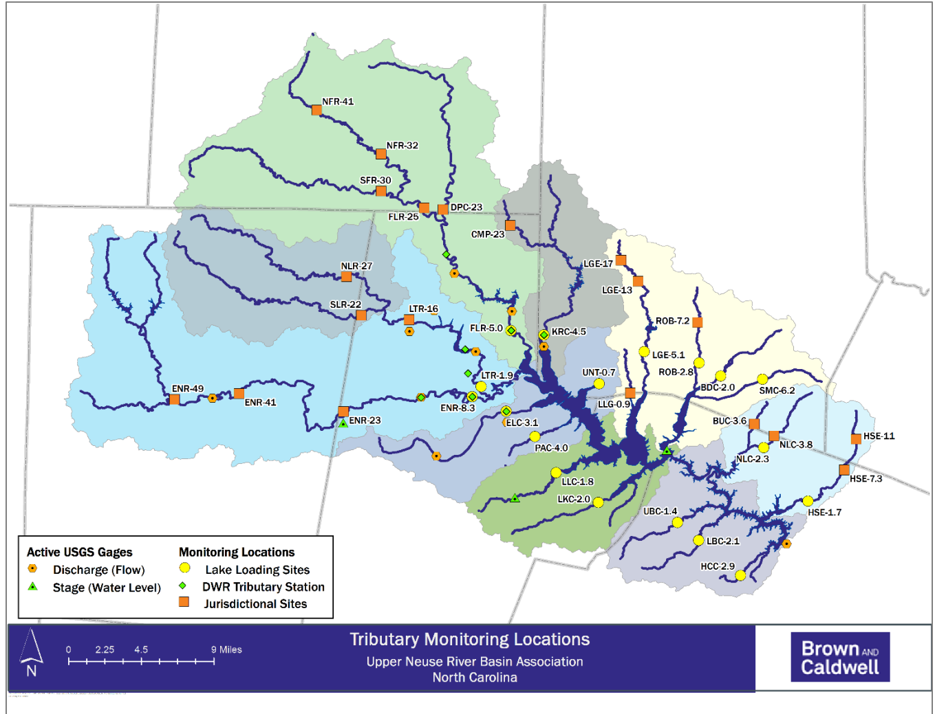
Figure G-1. Locations of sources of water quality data within the Falls Lake watershed
