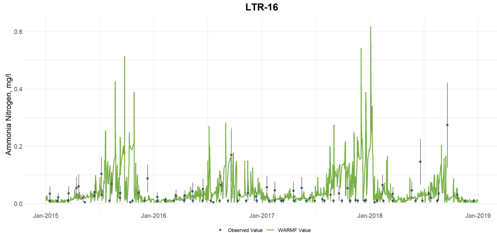
Figure G-67. Comparison of Observed and Simulated Ammonia Concentrations at Little River at Station LTR-16 (vertical bars are used to illustrate the uncertainty with laboratory analyses and are based on the 95th percentile confidence interval calculated from the UNRBA data set for each parameter)
