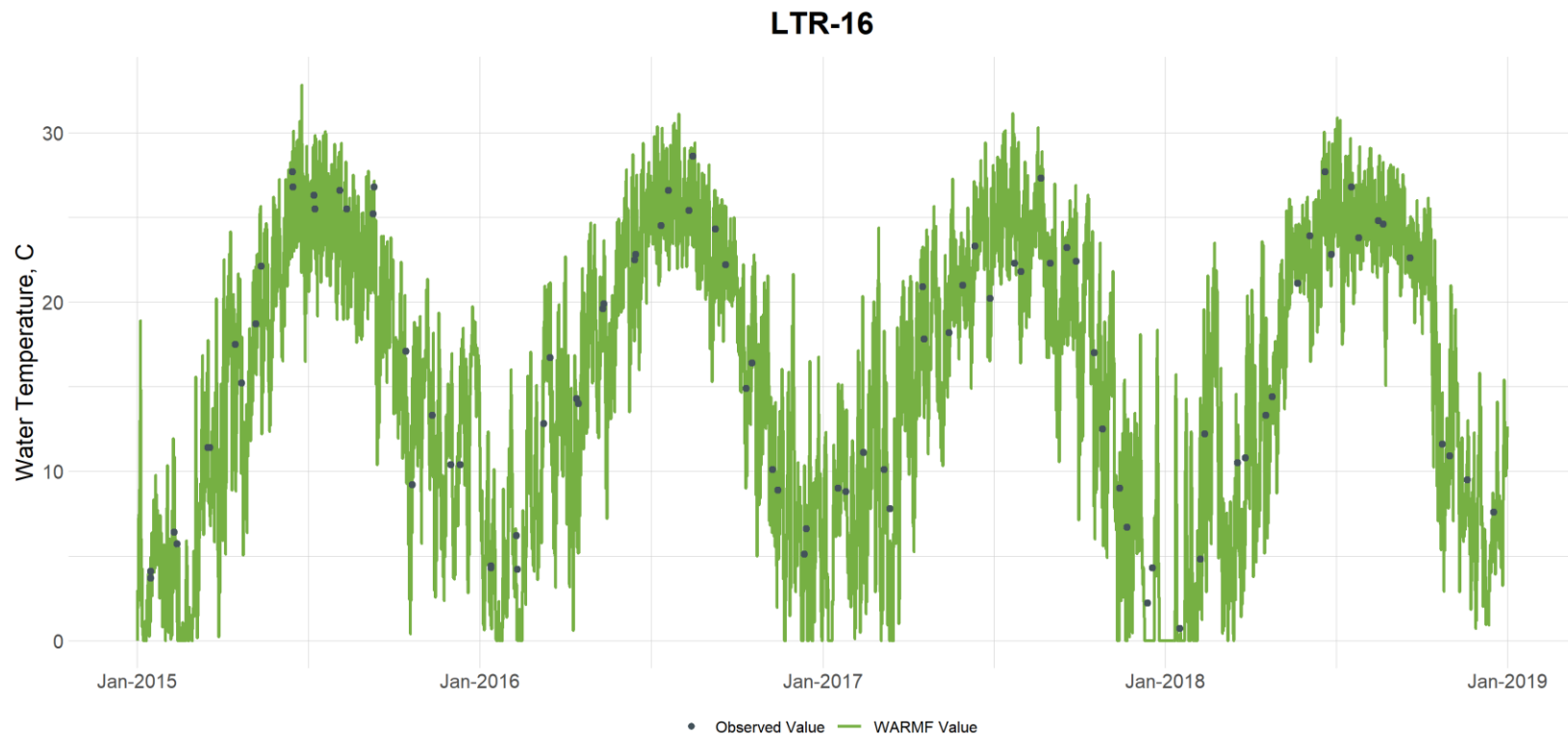
Figure G-66. Comparison of Observed and Simulated Stream Temperatures at Little River at Station LTR-16
