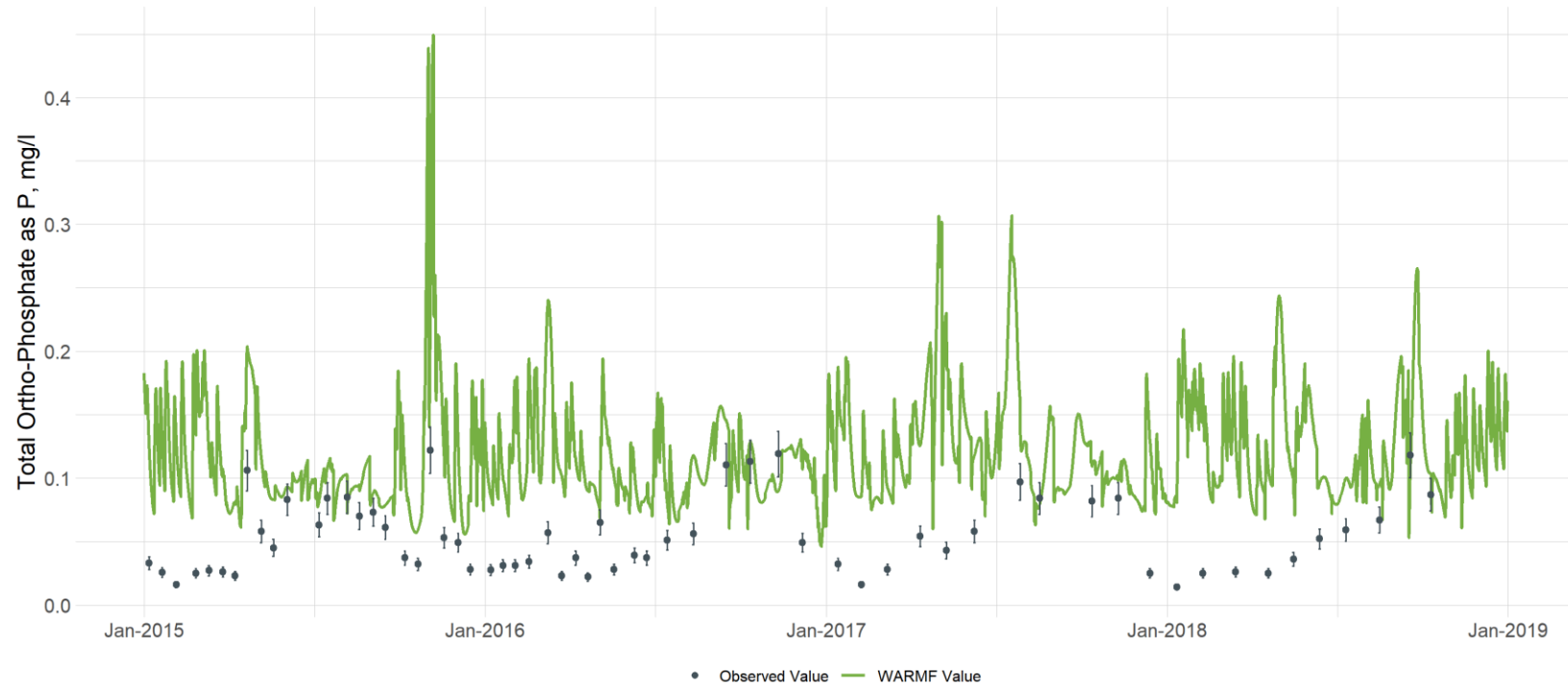
Figure G-11. Comparison of Observed and Simulated Total Ortho-Phosphate Concentrations at Ellerbe Creek at Station ELC-3.1 (vertical bars are used to illustrate the uncertainty with laboratory analyses and are based on the 95th percentile confidence interval calculated from the UNRBA data set for each parameter)
