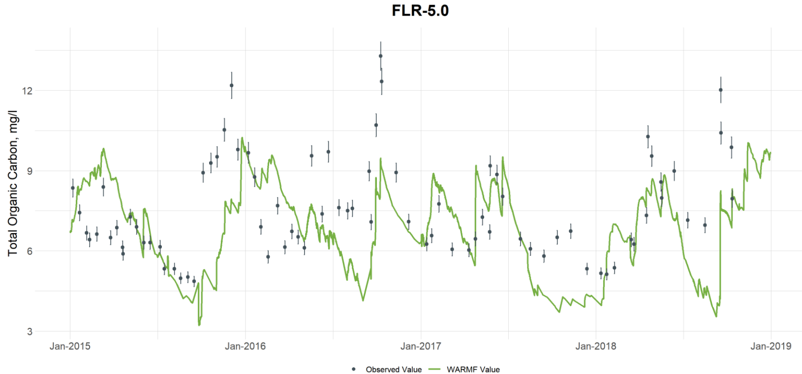
Figure G-49. Comparison of Observed and Simulated Total Organic Carbon Concentrations at Flat River at Station FLR-5 (downstream of Lake Michie) (vertical bars are used to illustrate the uncertainty with laboratory analyses and are based on the 95 th percentile confidence interval calculated from the UNRBA data set for each parameter)
