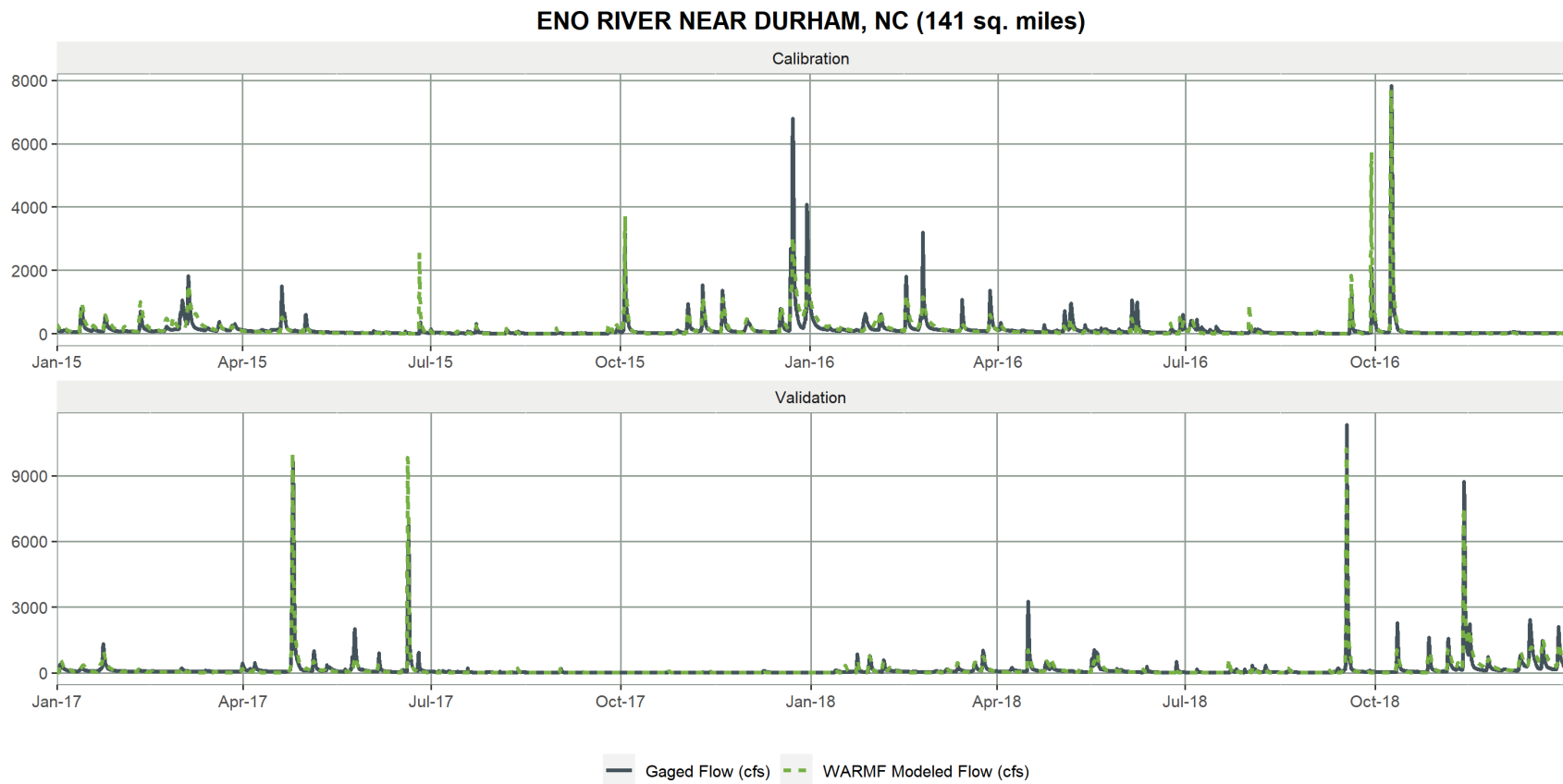
Figure G-15. Comparison of Observed and Simulated Stream Flows at Eno River near Durham, NC (141 square miles)
