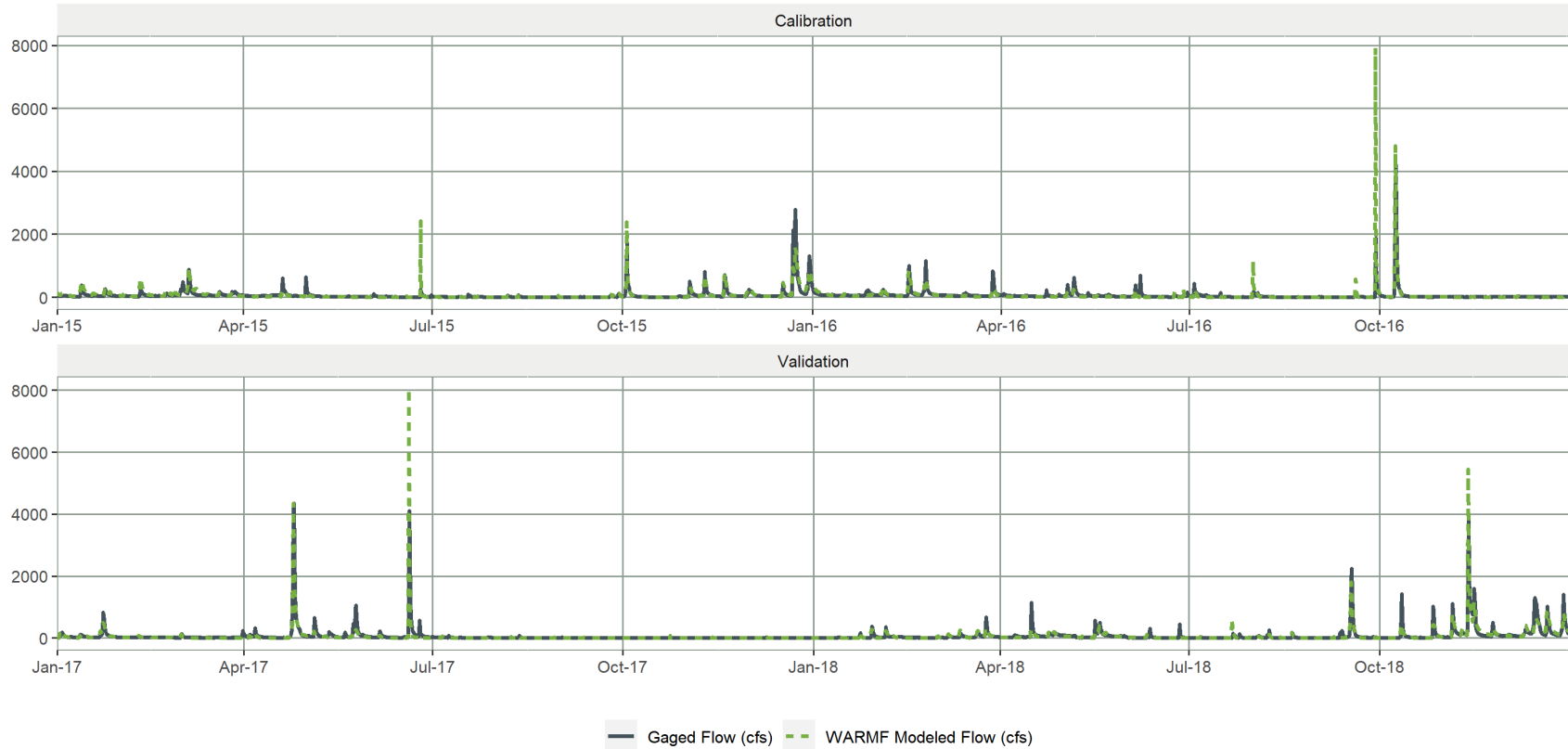
Figure G-14. Comparison of Observed and Simulated Stream Flows at Eno River at Hillsborough, NC (66 square miles)
