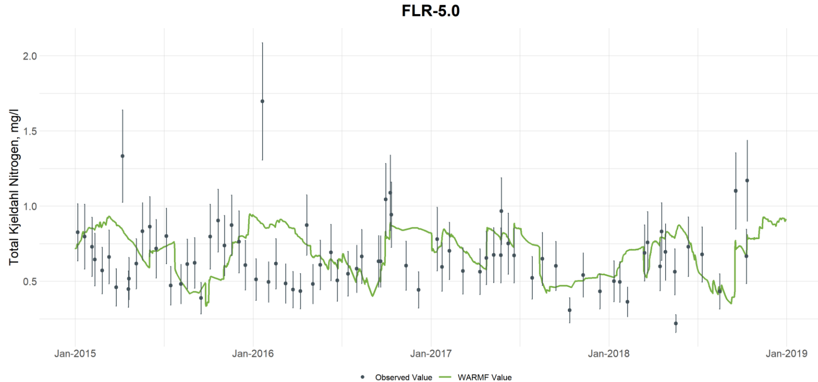
Figure G-47. Comparison of Observed and Simulated Total Kjeldahl Nitrogen Concentrations at Flat River at Station FLR-5 (downstream of Lake Michie) (vertical bars are used to illustrate the uncertainty with laboratory analyses and are based on the 95 th percentile confidence interval calculated from the UNRBA data set for each parameter)
