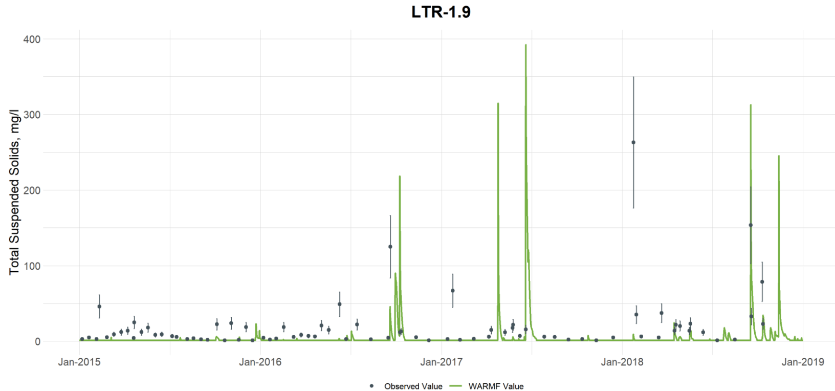
Figure G-82. Comparison of Observed and Simulated Total Suspended Solids (silt+clay) Concentrations at Little River at Station LTR-1.9 (downstream of Little River Reservoir) (vertical bars are used to illustrate the uncertainty with laboratory analyses and are based on the 95th percentile confidence interval calculated from the UNRBA data set for each parameter)
