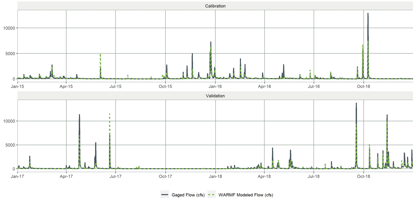
Figure G-34. Comparison of Observed and Simulated Stream Flows at Flat River at Bahama, NC (149 square miles)
