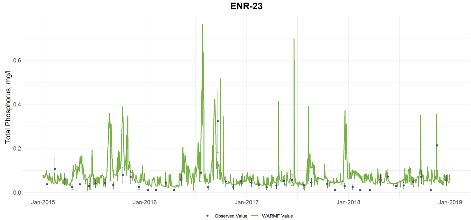
Figure G-22. Comparison of Observed and Simulated Total Phosphorus Concentrations at Eno River at Station ENR-23 (vertical bars are used to illustrate the uncertainty with laboratory analyses and are based on the 95th percentile confidence interval calculated from the UNRBA data set for each parameter)
