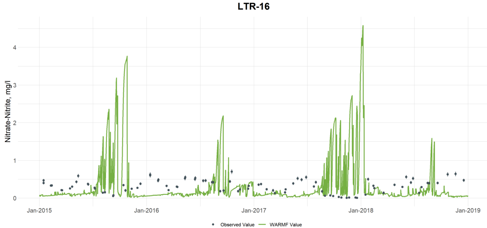
Figure G-68. Comparison of Observed and Simulated Nitrate-Nitrite Concentrations at Little River at Station LTR-16 (vertical bars are used to illustrate the uncertainty with laboratory analyses and are based on the 95th percentile confidence interval calculated from the UNRBA data set for each parameter)
