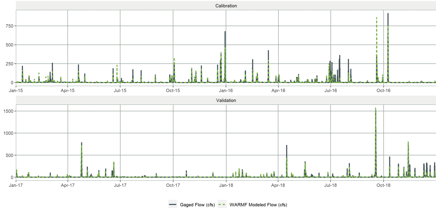
Figure G-2. Comparison of Observed and Simulated Stream Flows at Ellerbe Creek at Club Boulevard at Durham, NC (6.01 square miles)
