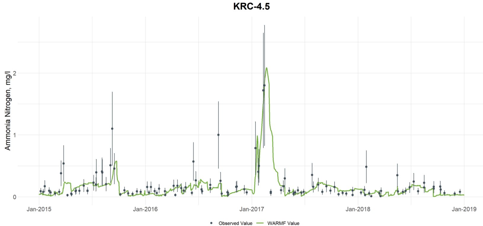
Figure G-56. Comparison of Observed and Simulated Ammonia Concentrations at Knap of Reeds Creek at Station KRC-4.5 (vertical bars are used to illustrate the uncertainty with laboratory analyses and are based on the 95th percentile confidence interval calculated from the UNRBA data set for each parameter)
