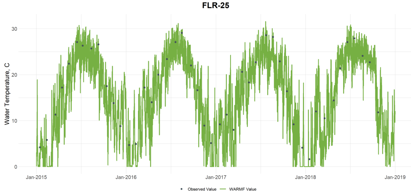
Figure G-36. Comparison of Observed and Simulated Stream Temperatures at Flat River at Station FLR-25
