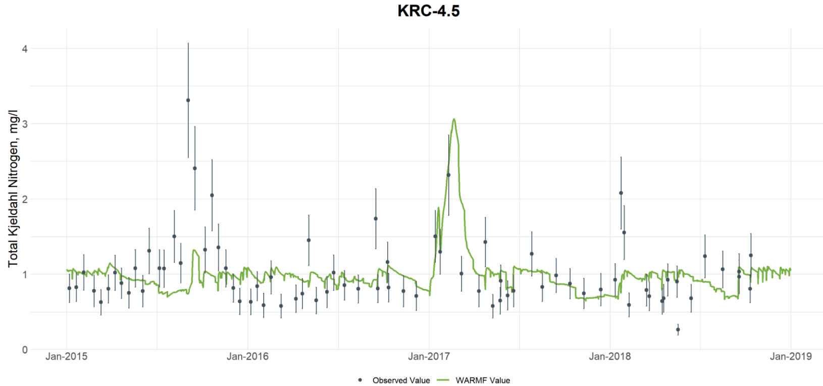
Figure G-58. Comparison of Observed and Simulated Total Kjeldahl Nitrogen Concentrations at Knap of Reeds Creek at Station KRC-4.5 (vertical bars are used to illustrate the uncertainty with laboratory analyses and are based on the 95th percentile confidence interval calculated from the UNRBA data set for each parameter)
