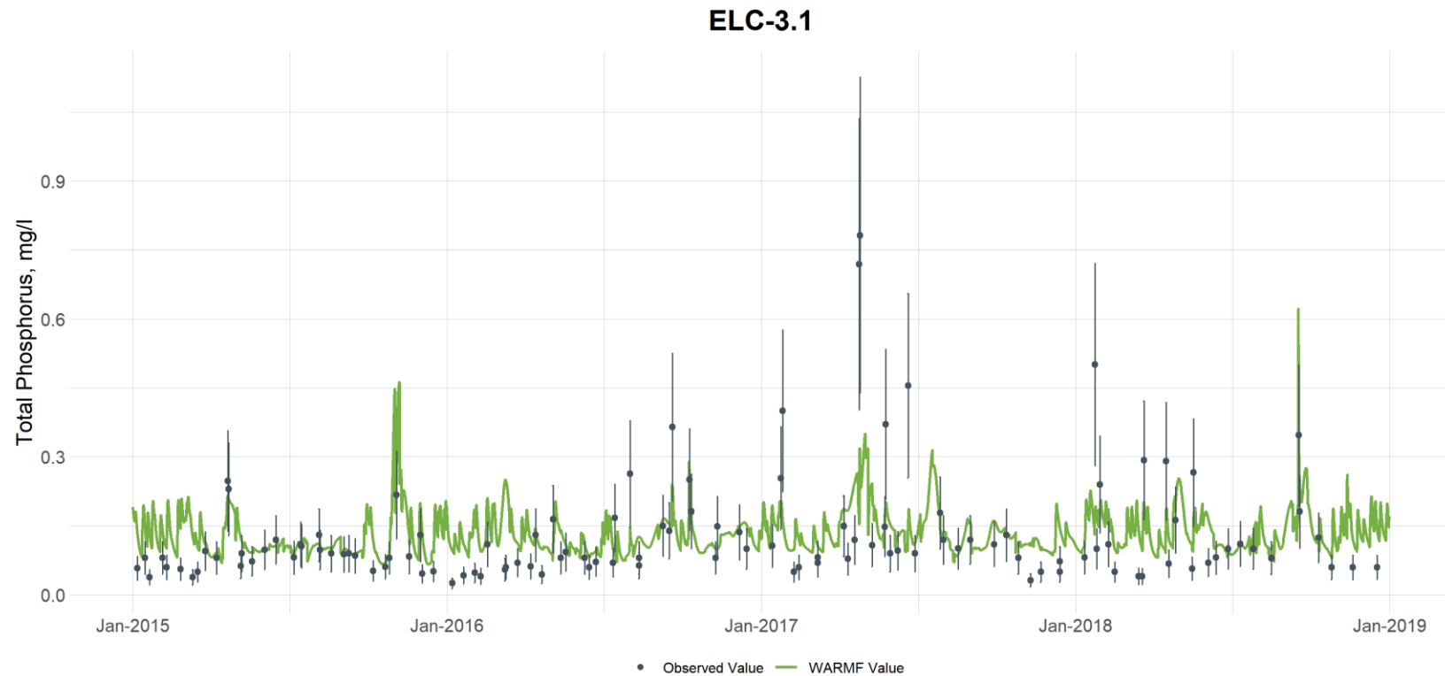
Figure G-10. Comparison of Observed and Simulated Total Phosphorus Concentrations at Ellerbe Creek at Station ELC-3.1 (vertical bars are used to illustrate the uncertainty with laboratory analyses and are based on the 95th percentile confidence interval calculated from the UNRBA data set for each parameter)
