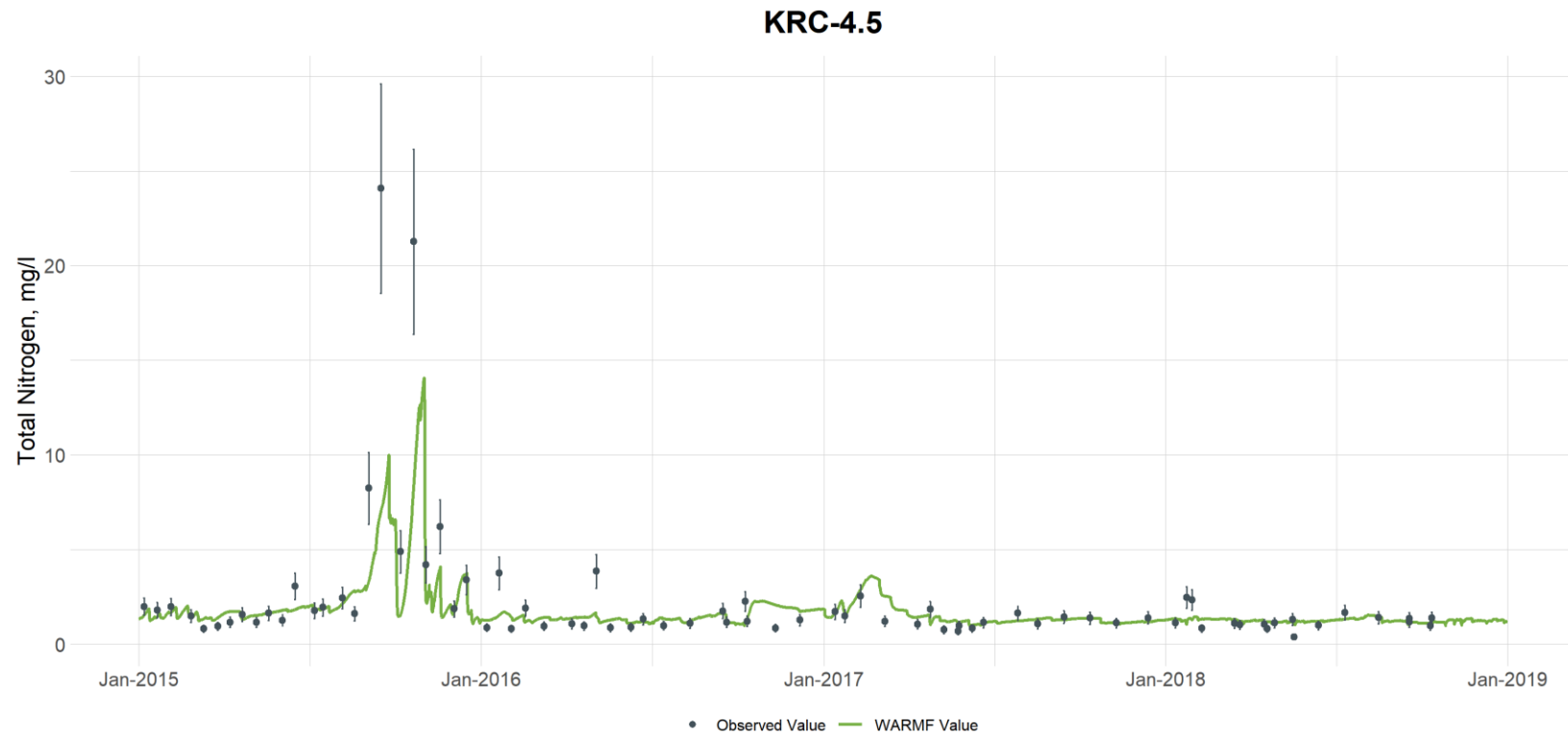
Figure G-59. Comparison of Observed and Simulated Total Nitrogen Concentrations at Knap of Reeds Creek at Station KRC-4.5 (vertical bars are used to illustrate the uncertainty with laboratory analyses and are based on the 95th percentile confidence interval calculated from the UNRBA data set for each parameter)
