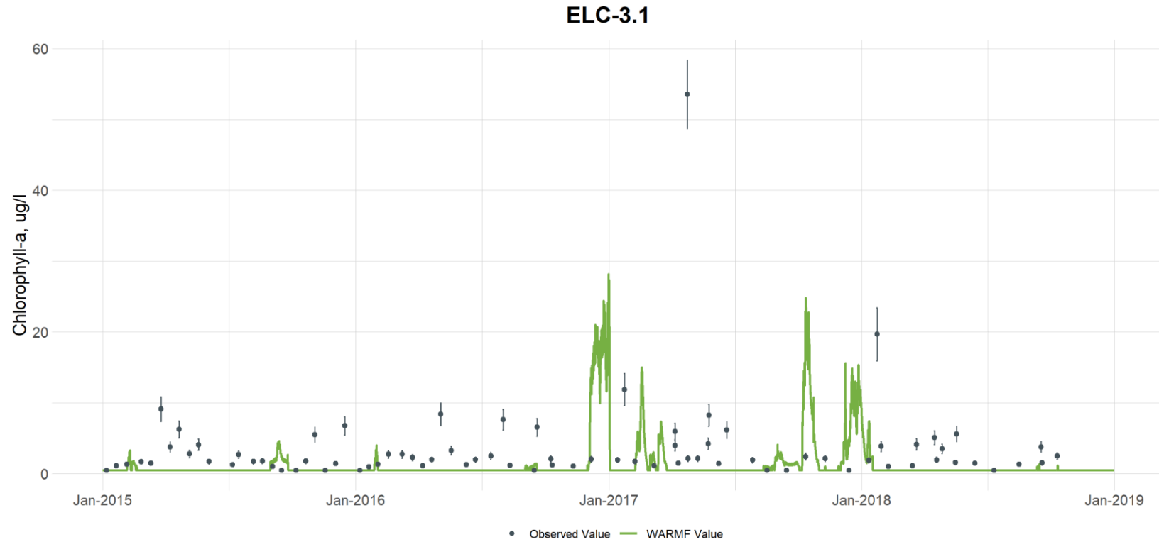
Figure G-13. Comparison of Observed and Simulated Chlorophyll-a Concentrations at Ellerbe Creek at Station ELC-3.1 (vertical bars are used to illustrate the uncertainty with laboratory analyses and are based on the 95th percentile confidence interval calculated from the UNRBA data set for each parameter)
