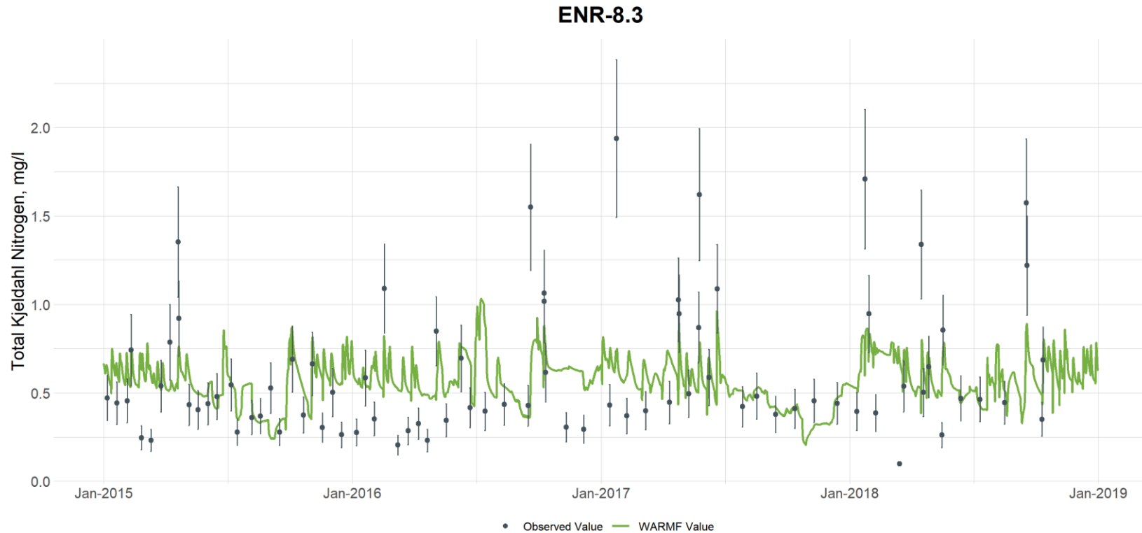
Figure G-27. Comparison of Observed and Simulated Total Kjeldahl Nitrogen Concentrations at Eno River at Station ENR-8.3 (vertical bars are used to illustrate the uncertainty with laboratory analyses and are based on the 95th percentile confidence interval calculated from the UNRBA data set for each parameter)
