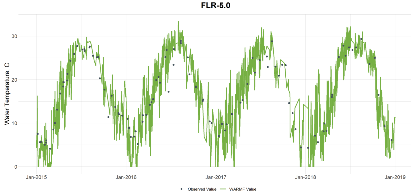
Figure G-44. Comparison of Observed and Simulated Stream Temperatures at Flat River at Station FLR-5 (downstream of Lake Michie)
