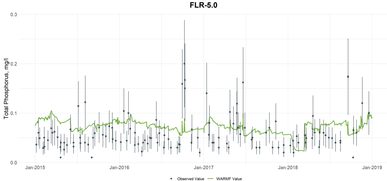
Figure G-50. Comparison of Observed and Simulated Total Phosphorus Concentrations at Flat River at Station FLR-5 (downstream of Lake Michie) (vertical bars are used to illustrate the uncertainty with laboratory analyses and are based on the 95 th percentile confidence interval calculated from the UNRBA data set for each parameter)
