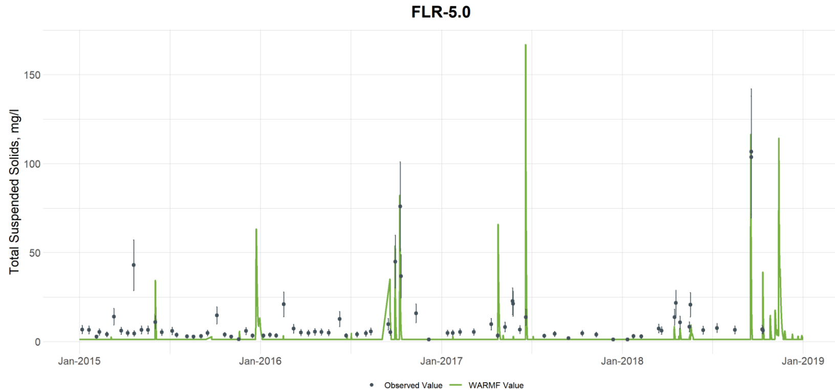
Figure G-52. Comparison of Observed and Simulated Total Suspended Solids (silt+clay) Concentrations at Flat River at Station FLR-5 (downstream of Lake Michie) (vertical bars are used to illustrate the uncertainty with laboratory analyses and are based on the 95th percentile confidence interval calculated from the UNRBA data set for each parameter)
