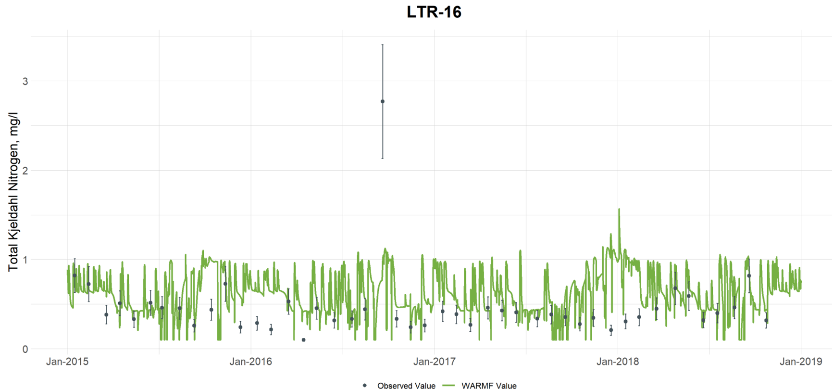
Figure G-69. Comparison of Observed and Simulated Total Kjeldahl Nitrogen Concentrations at Little River at Station LTR-16 (vertical bars are used to illustrate the uncertainty with laboratory analyses and are based on the 95th percentile confidence interval calculated from the UNRBA data set for each parameter)
