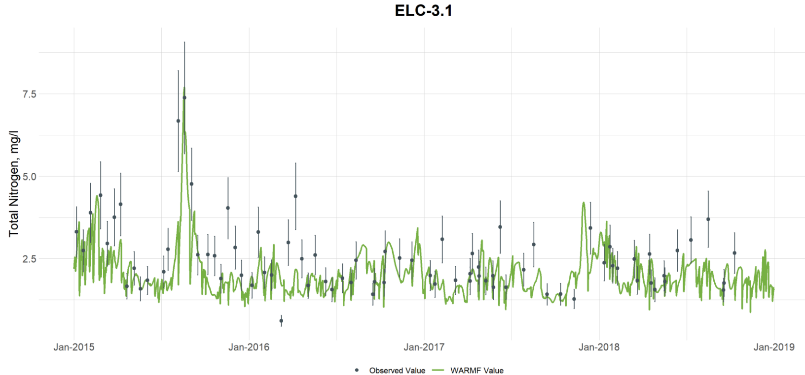
Figure G-8. Comparison of Observed and Simulated Total Nitrogen Concentrations at Ellerbe Creek at Station ELC-3.1 (vertical bars are used to illustrate the uncertainty with laboratory analyses and are based on the 95th percentile confidence interval calculated from the UNRBA data set for each parameter)
