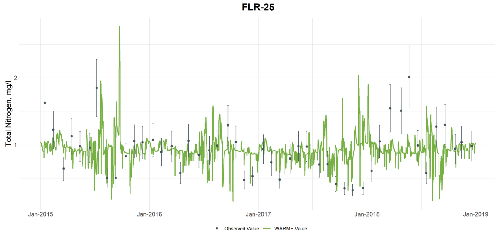
Figure G-40. Comparison of Observed and Simulated Total Nitrogen Concentrations at Flat River at Station FLR-25 (vertical bars are used to illustrate the uncertainty with laboratory analyses and are based on the 95 th percentile confidence interval calculated from the UNRBA data set for each parameter)
