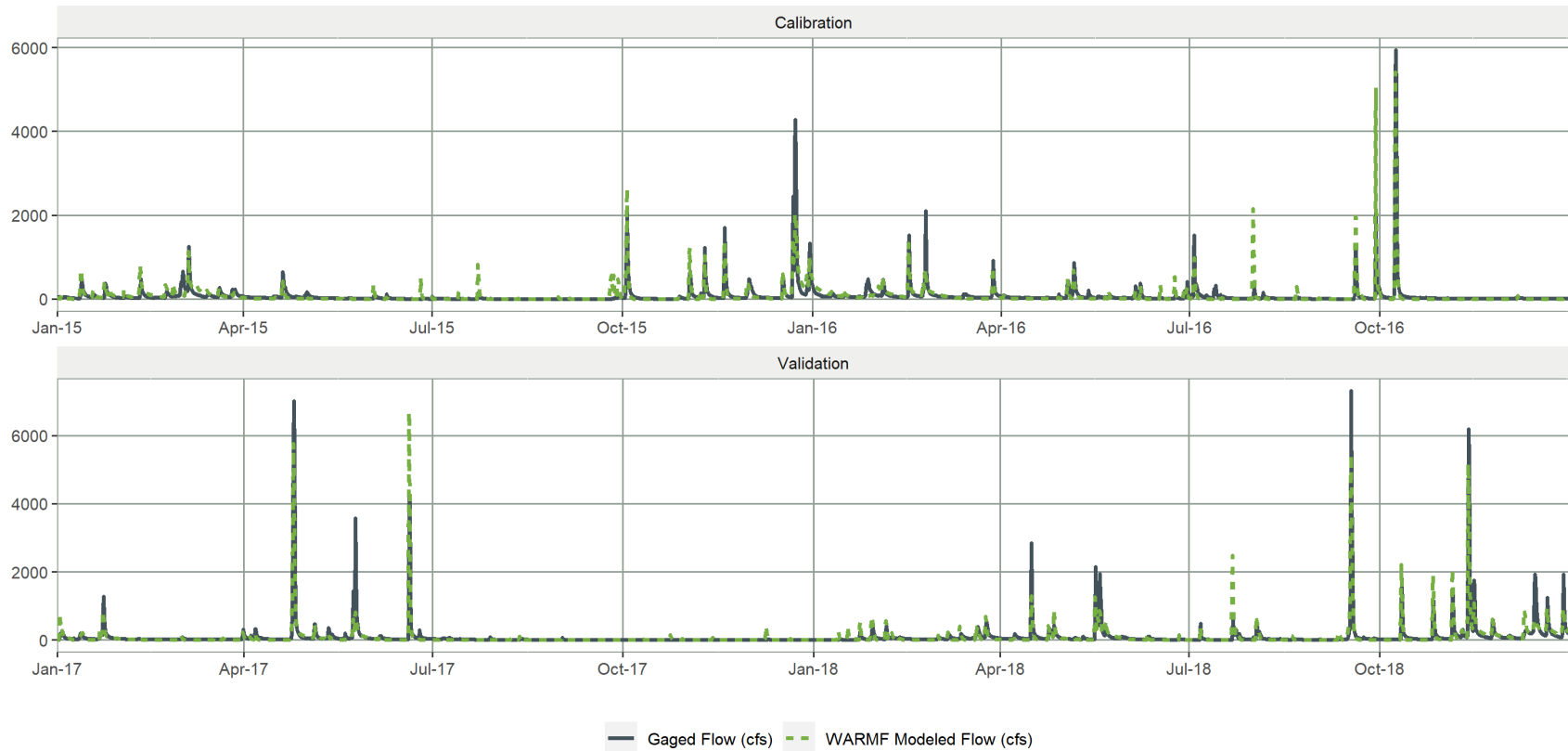
Figure G-65. Comparison of Observed and Simulated Stream Flows at Little River at SR1461 near Orange Factory, NC (78.2 square miles)
