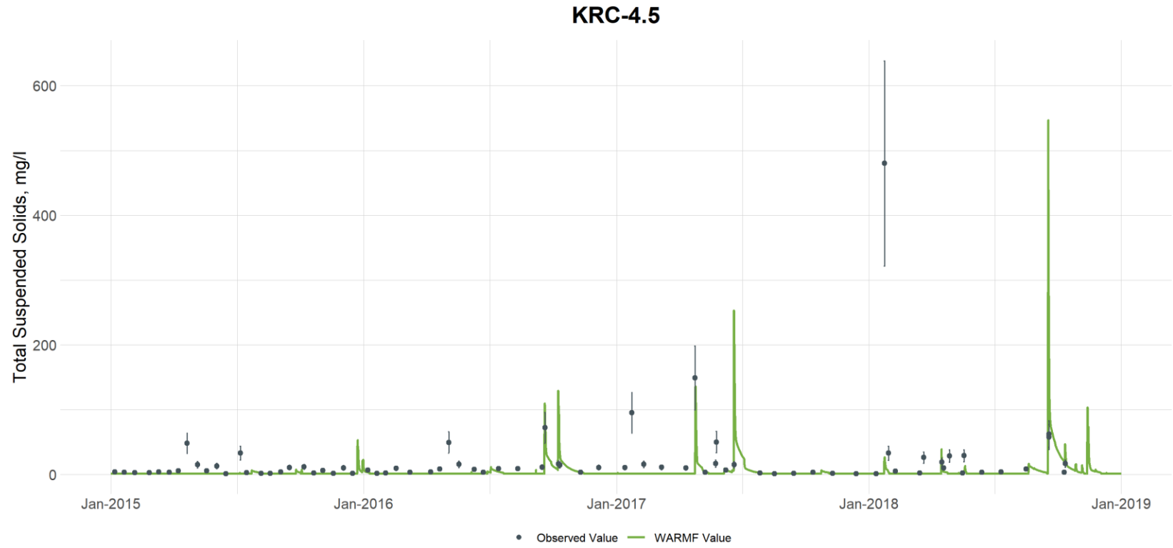
Figure G-63. Comparison of Observed and Simulated Total Suspended Solids (silt+clay) Concentrations at Knap of Reeds Creek at Station KRC-4.5 (vertical bars are used to illustrate the uncertainty with laboratory analyses and are based on the 95th percentile confidence interval calculated from the UNRBA data set for each parameter)
