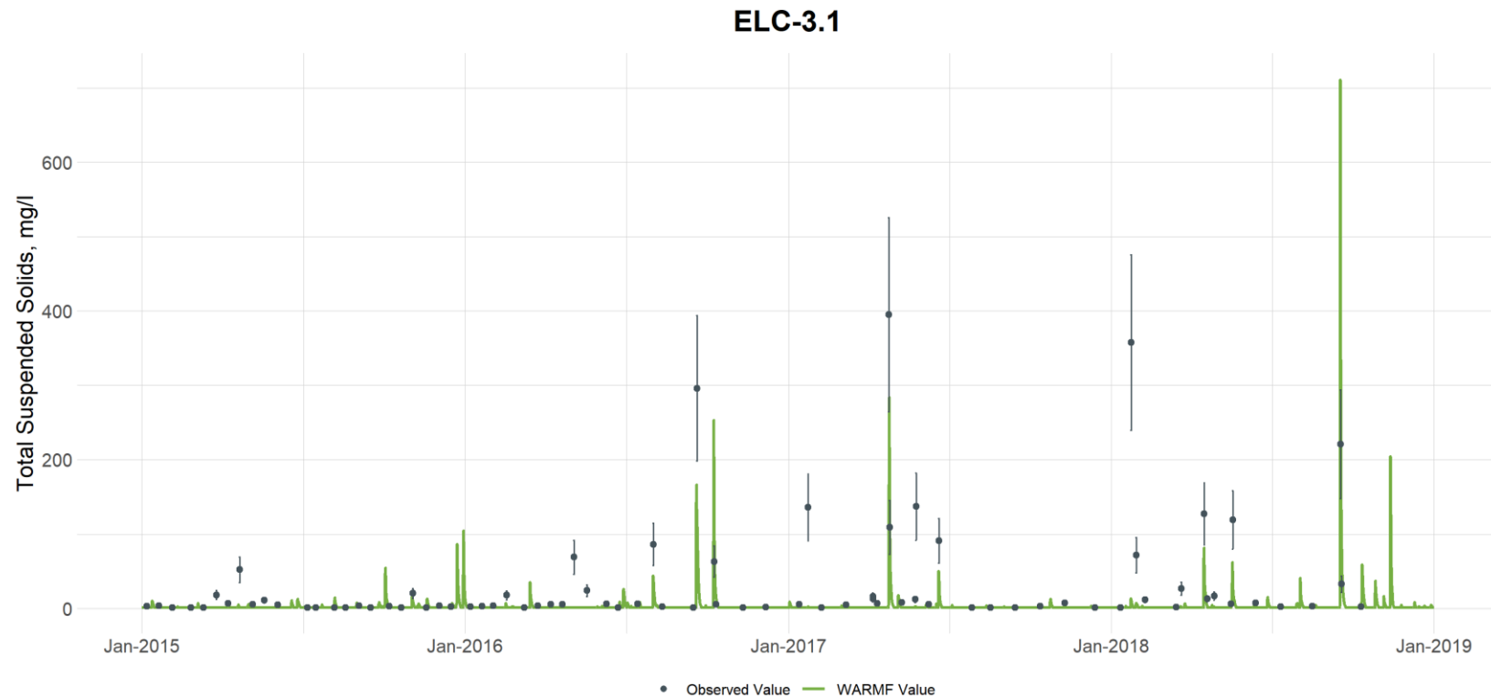
Figure G-12. Comparison of Observed and Simulated Total Suspended Solids (silt+clay) Concentrations at Ellerbe Creek at Station ELC-3.1 (vertical bars are used to illustrate the uncertainty with laboratory analyses and are based on the 95th percentile confidence interval calculated from the UNRBA data set for each parameter)
