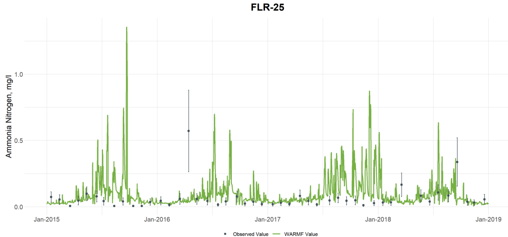
Figure G-37. Comparison of Observed and Simulated Ammonia Concentrations at Flat River at Station FLR-25 (vertical bars are used to illustrate the uncertainty with laboratory analyses and are based on the 95 th percentile confidence interval calculated from the UNRBA data set for each parameter)
