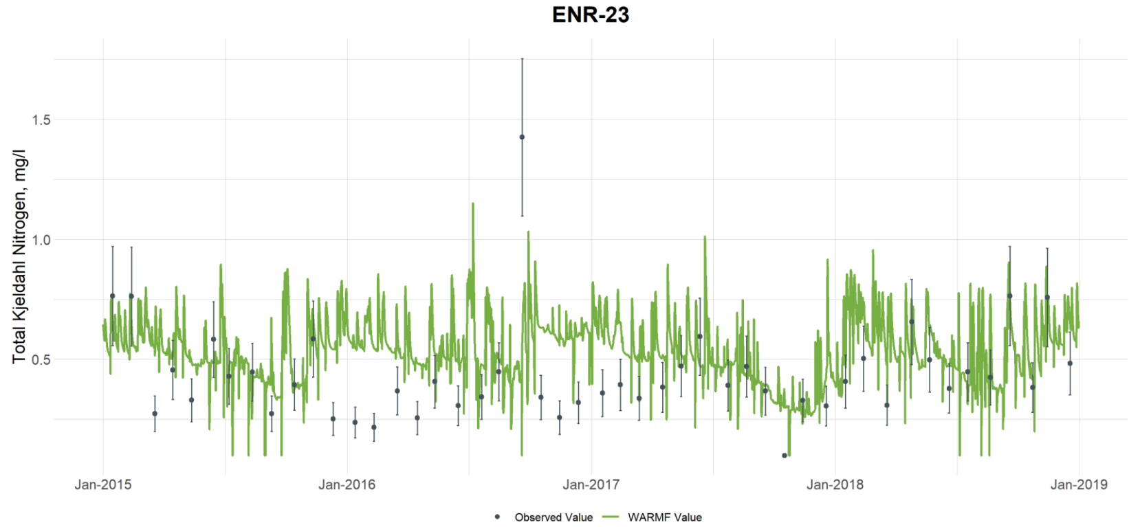
Figure G-19. Comparison of Observed and Simulated Total Kjeldahl Nitrogen Concentrations at Eno River at Station ENR-23 (vertical bars are used to illustrate the uncertainty with laboratory analyses and are based on the 95th percentile confidence interval calculated from the UNRBA data set for each parameter)
