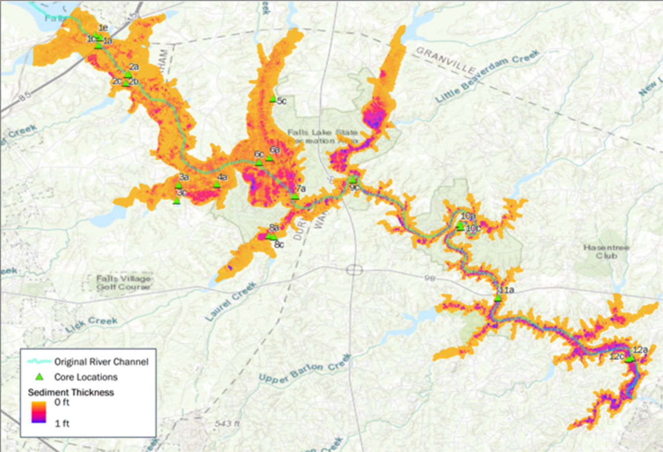
Falls Lake Sediment Thickness Upper Neuse River Basin Association North Carolina
